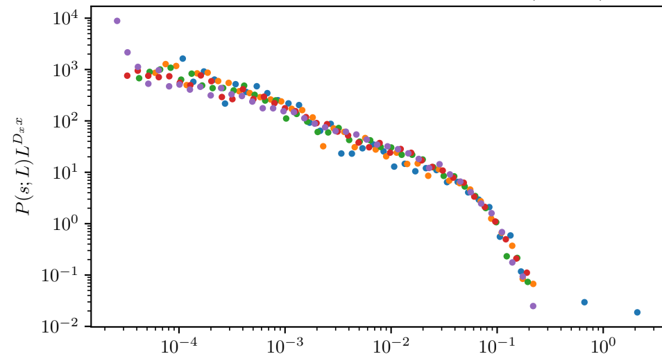
Affine initial-guess energy pre: x=0.848 , D=0.293 , x_{\min}=9.92\text{e-}06 ( L=250 )
