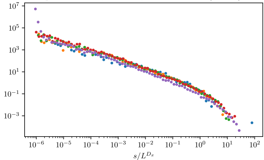
Affine initial-guess energy post: x=1.530 , D=0.287 , x_{\min}=4.05\text{e-}06 ( L=250 )
