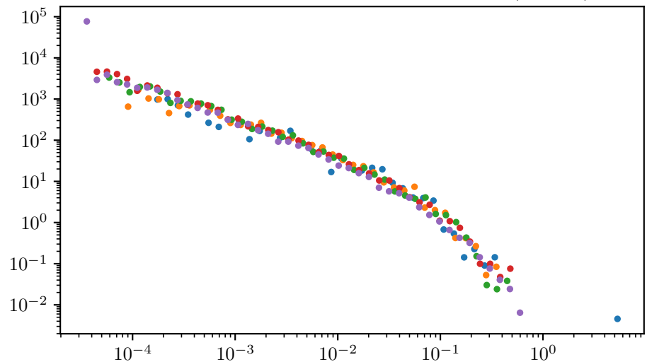
First-order elastic continuation post: x=1.240 , D=0.682 , x_{\min}=6.82\text{e-}03 ( L=250 )
