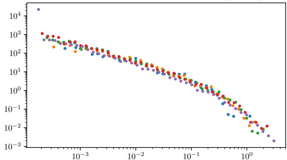
Previous relaxed energy post: x=1.152 , D=0.600 , x_{\min}=5.71\text{e-}01 ( L=250 )
