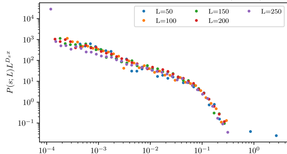
First-order elastic continuation pre: x=1.197 , D=0.795 , x_{\min}=8.75\text{e-}03 ( L=250 )
