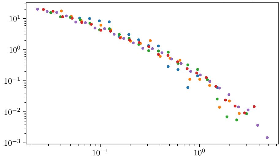
Affine initial-guess energy post: x=1.530 , D=0.287 , x_{\min}=4.05\text{e-}06 ( L=250 )
