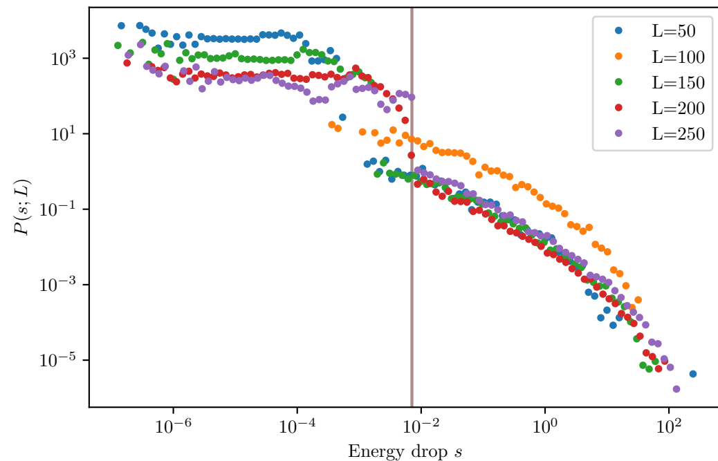
Second-order elastic continuation - post-yield Shared xmin=7.096e-03 from L=250 (slope)
