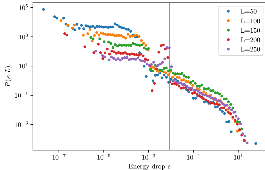
Second-order elastic continuation - pre-yield Shared xmin=8.565e-03 from L=250 (slope)
