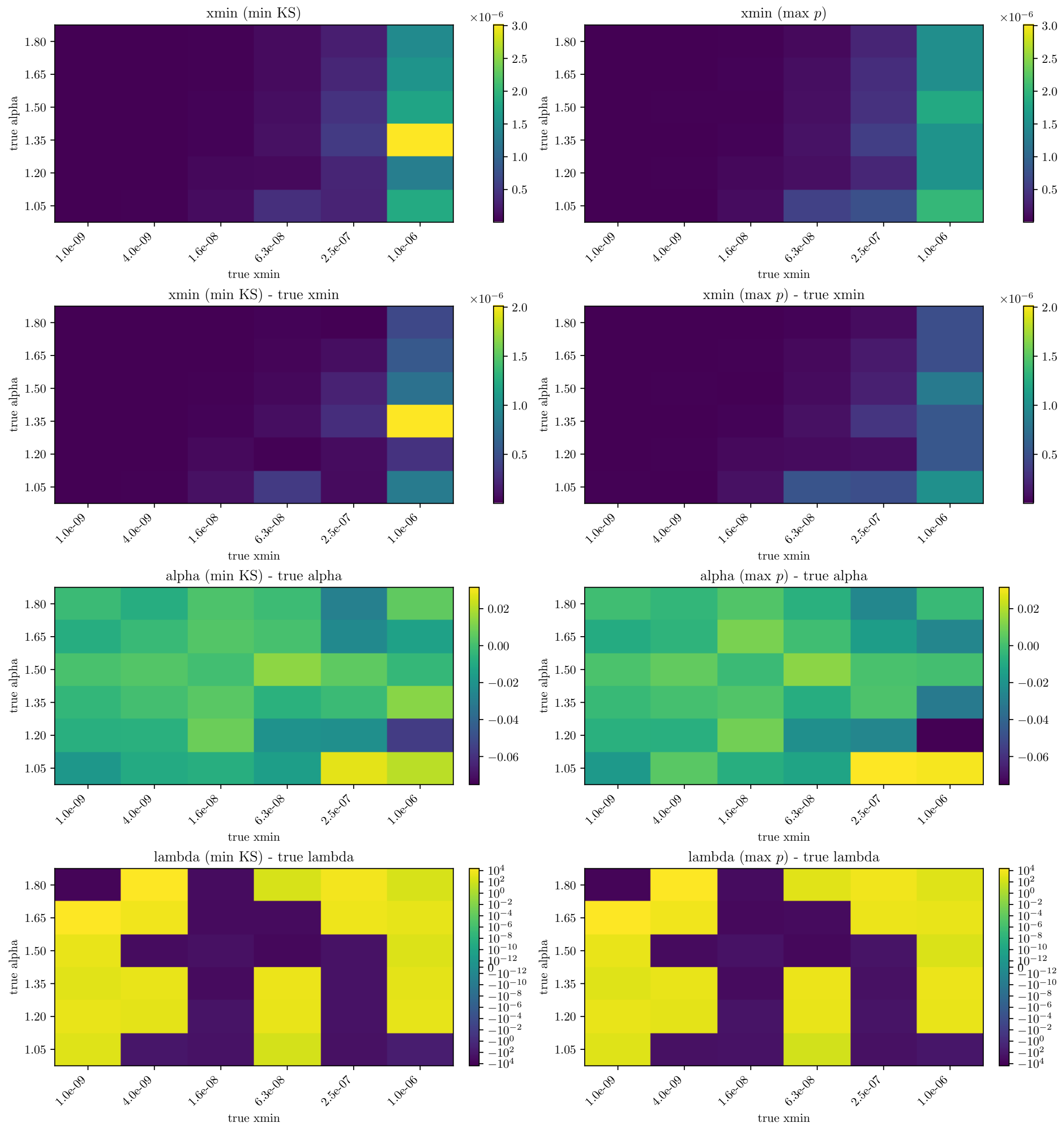
Grid comparison of xmin estimates
