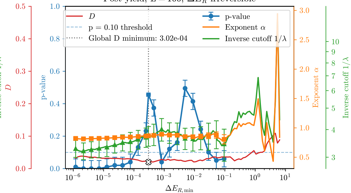
Post-yield, L = 100 ; \Delta E_R irreversible
