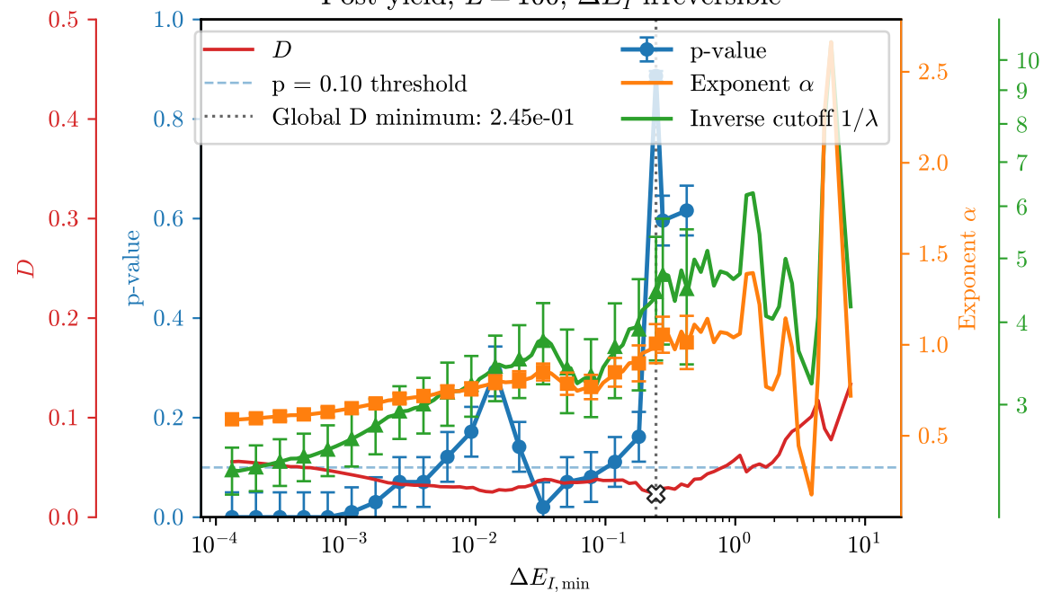
Post-yield, L = 100 ; \Delta E_I irreversible
