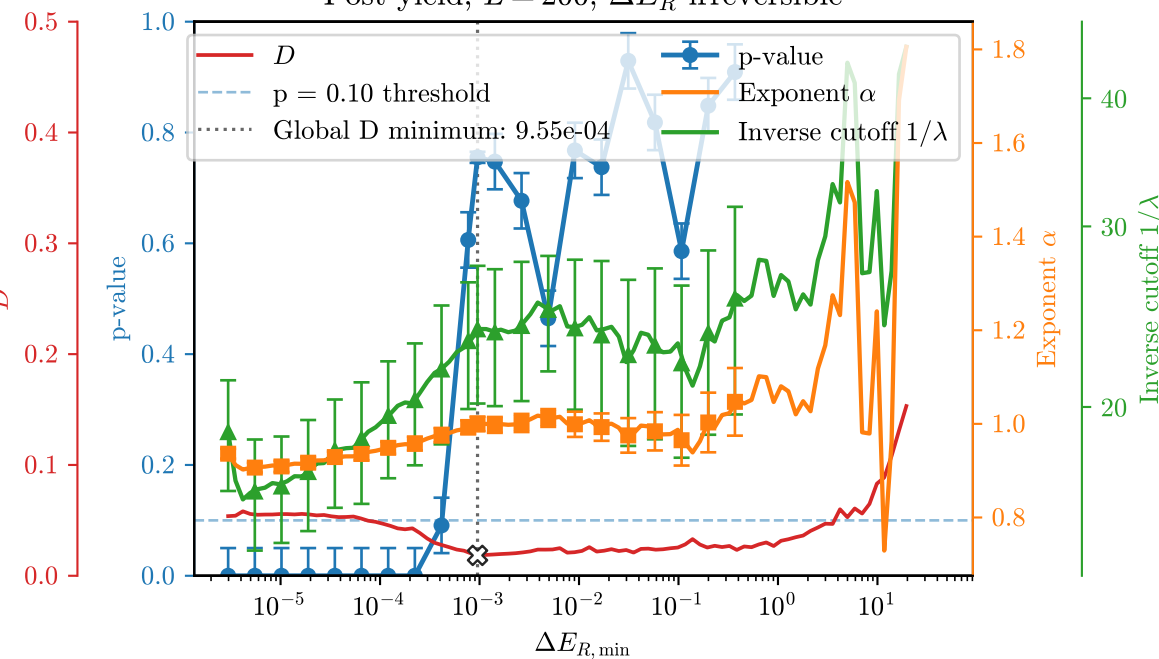
Post-yield, L = 200 ; \Delta E_R irreversible
