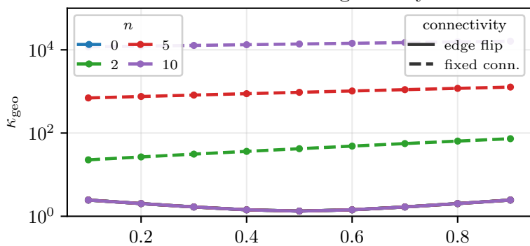
distorted current geometry
