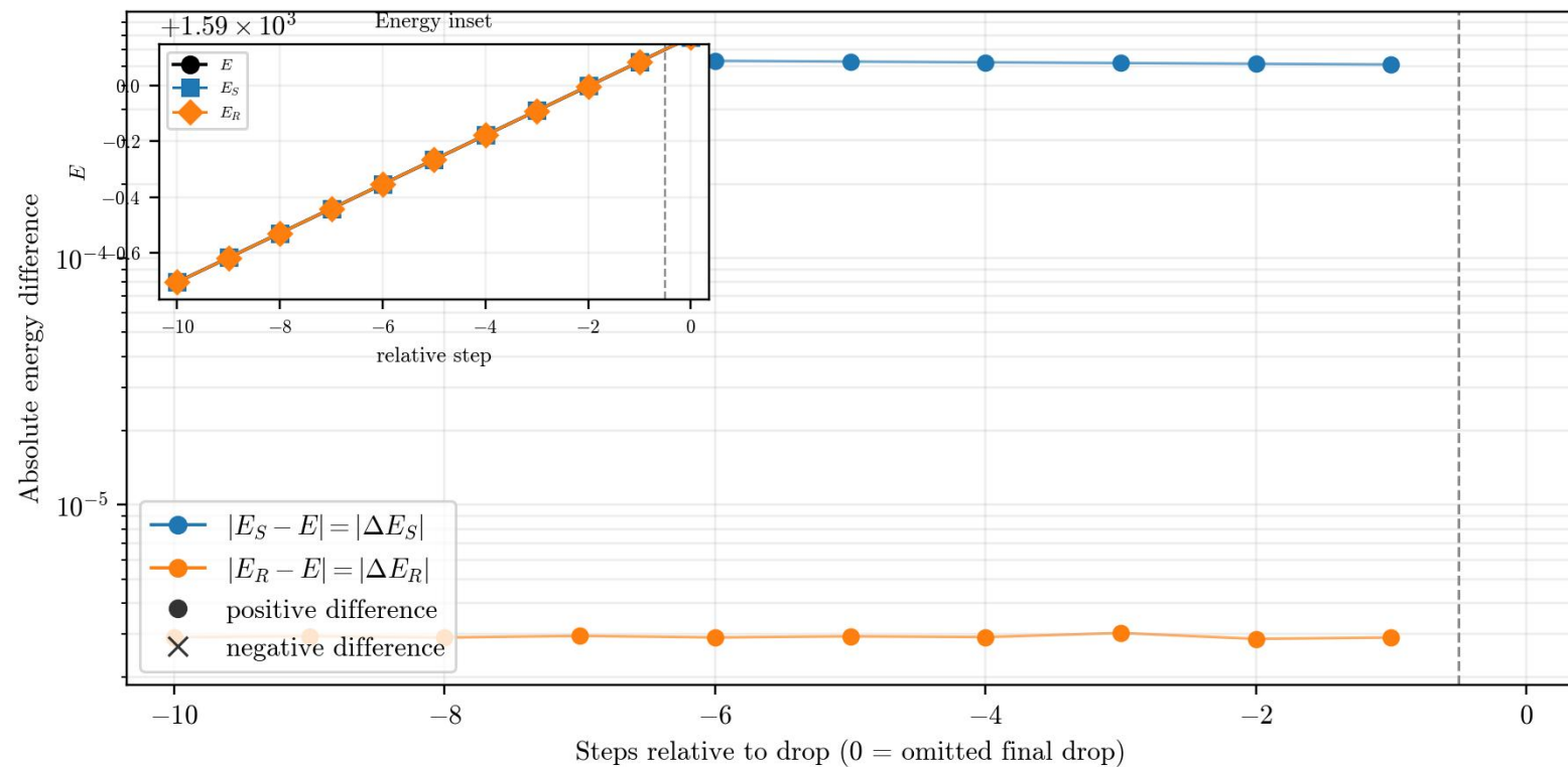
250x250 non-reconnecting energy-drop zoom reversible sample 3/20, load=0.62457, yield load=0.53102 \Delta E_S=0.000604268 , \Delta E_R=2.90297\text{e-}06 shared \Delta E_S \in [0.000417, 0.0144] , \kappa_{\text{det}}=3.04
