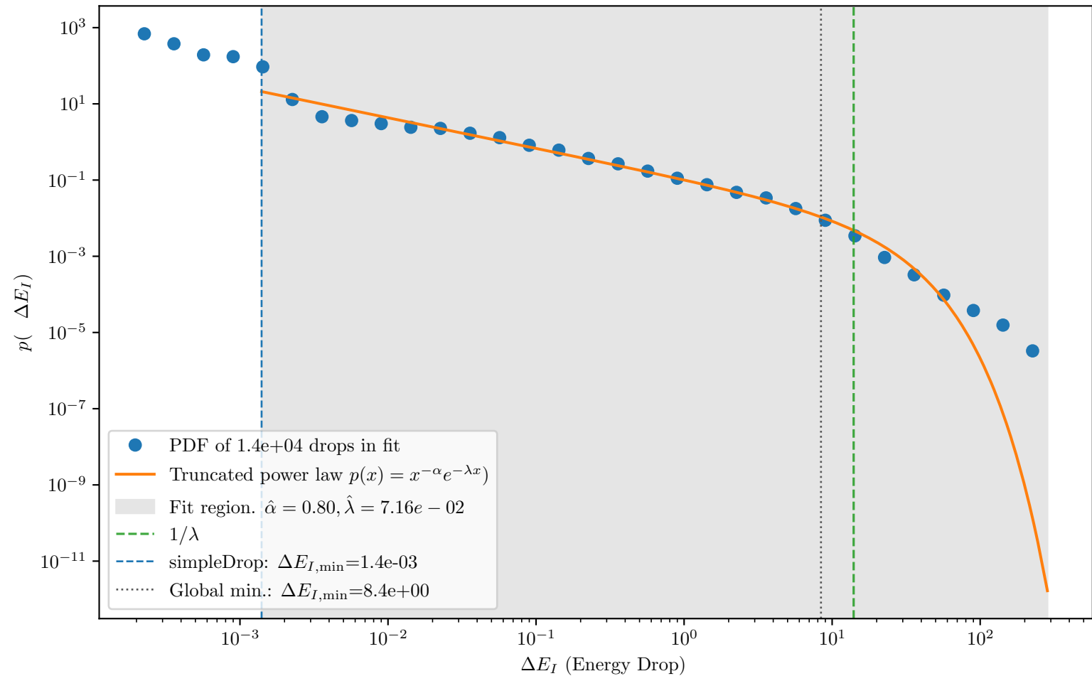
CG, L=100: E_I PDF with truncated-power-law fit
