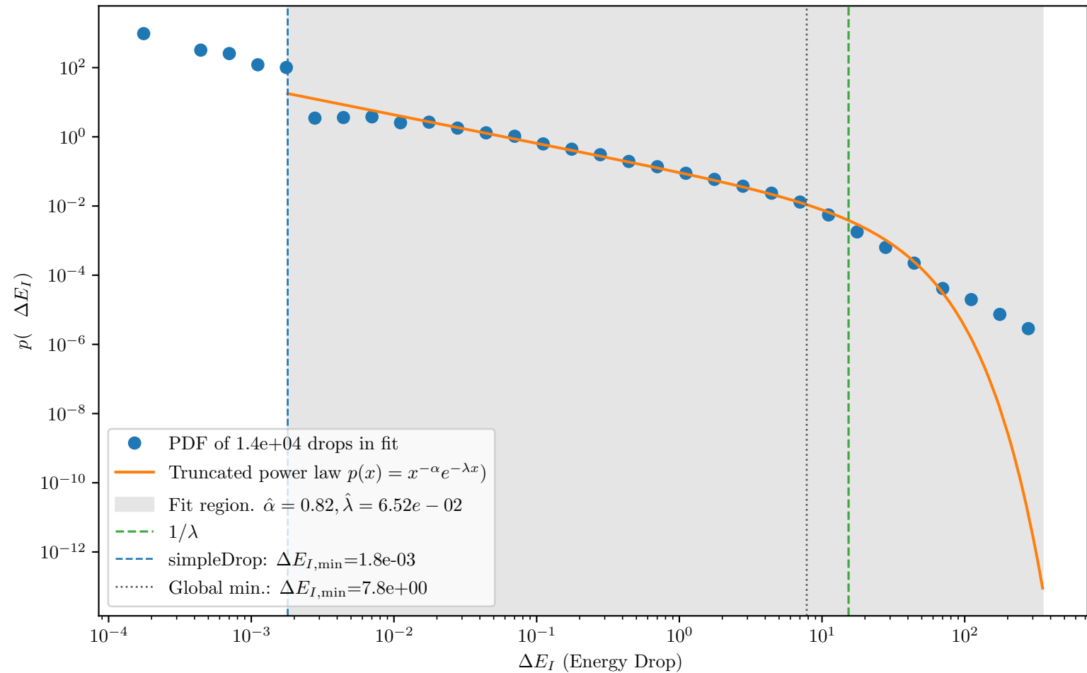
LBFGS, L=100: E_I PDF with truncated-power-law fit
