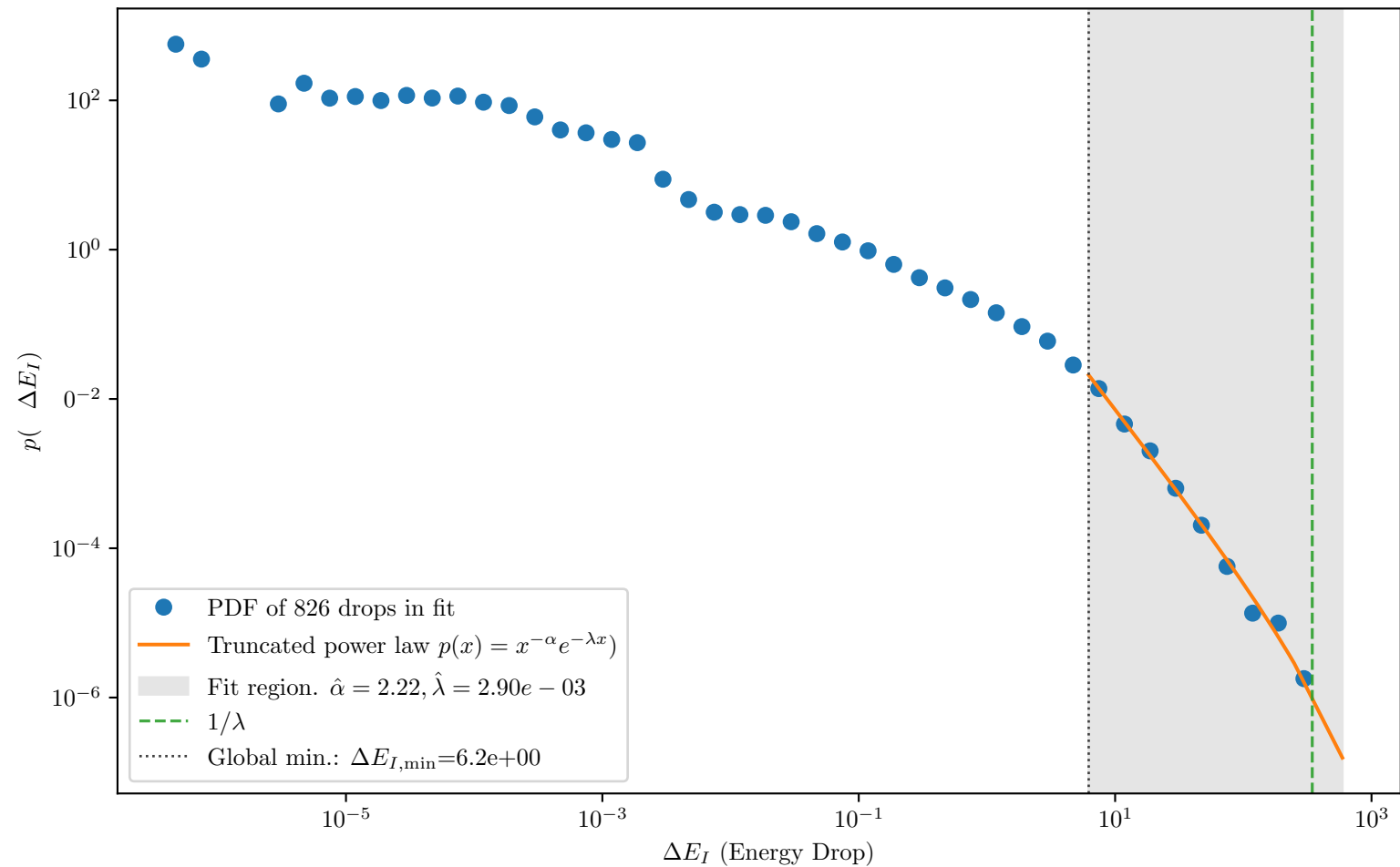
CG, L=200: E_I PDF with truncated-power-law fit
