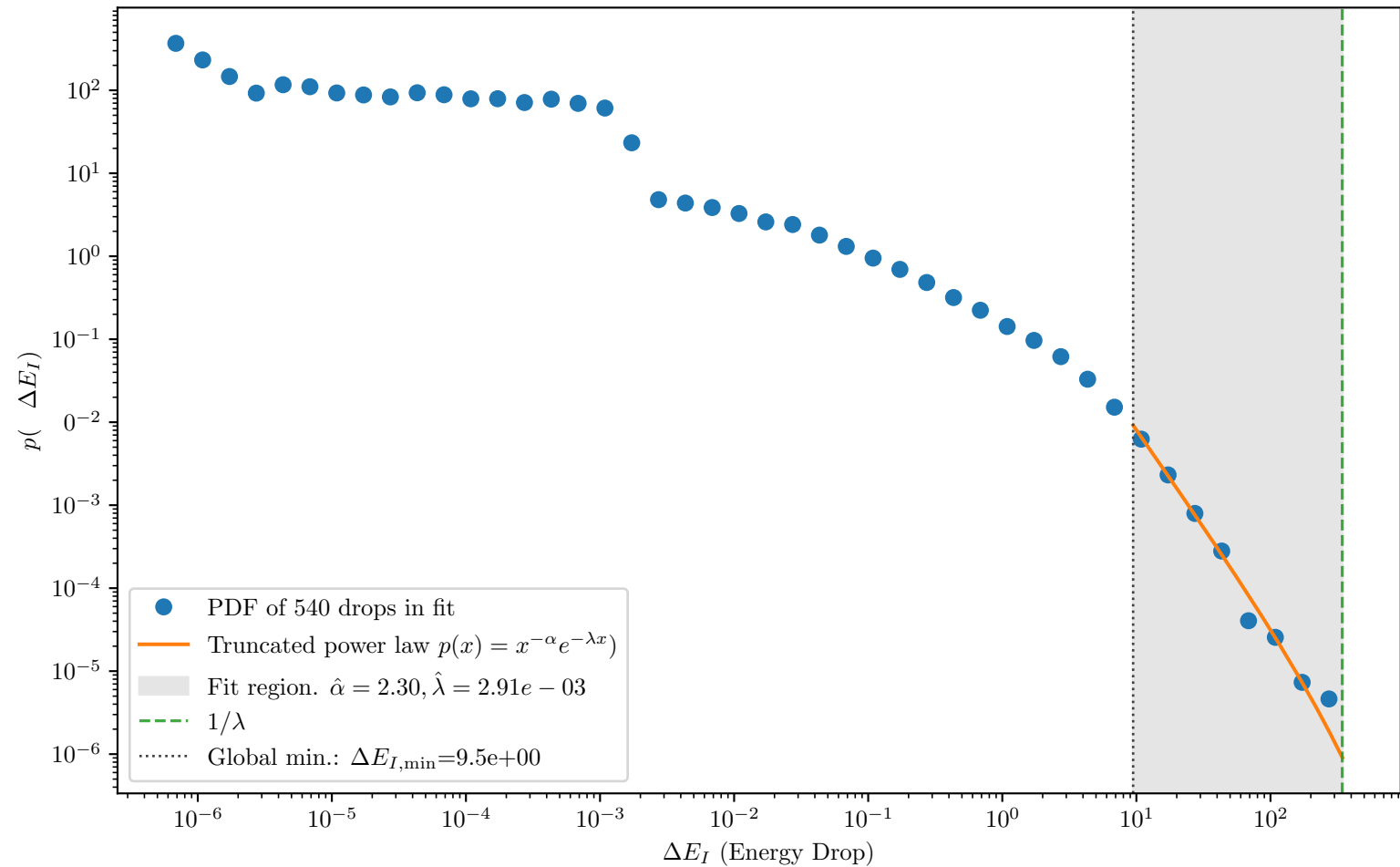
FIRE, L=200: E_I PDF with truncated-power-law fit
