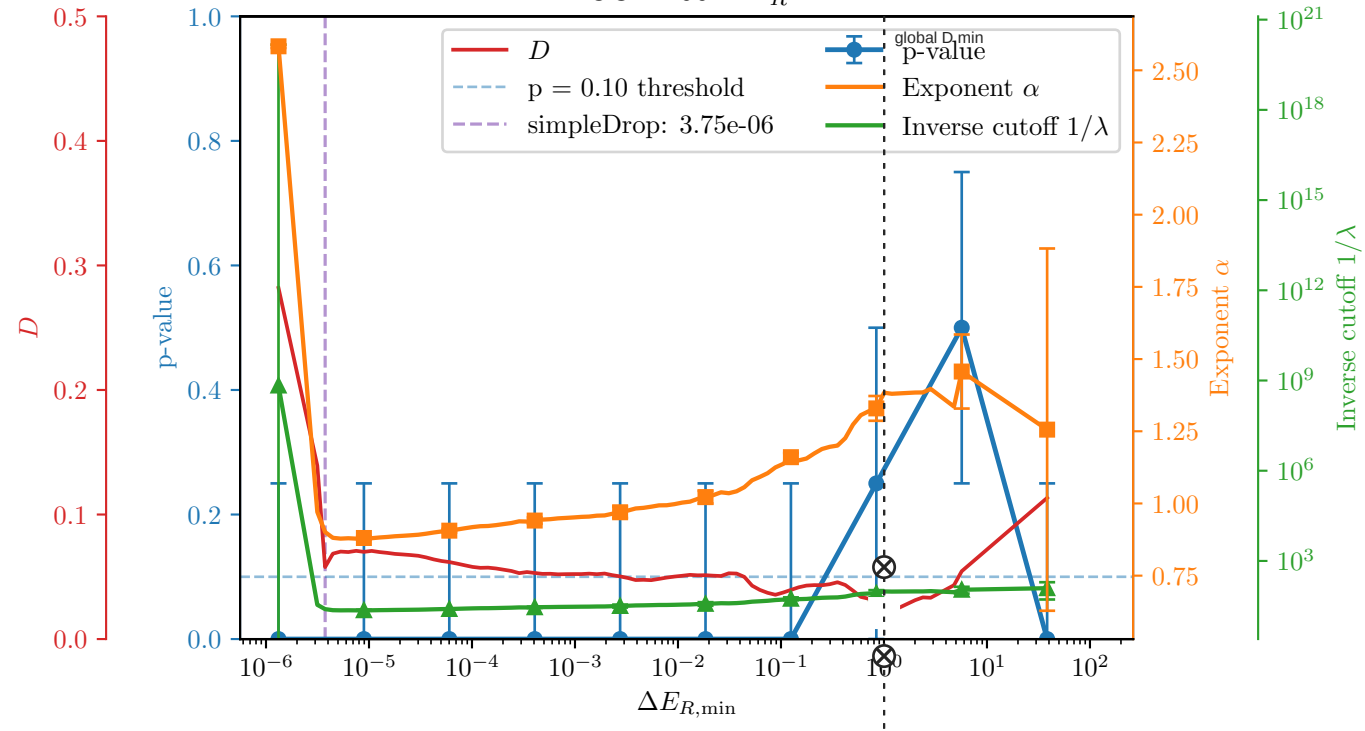
CG L200 \Delta E_R
