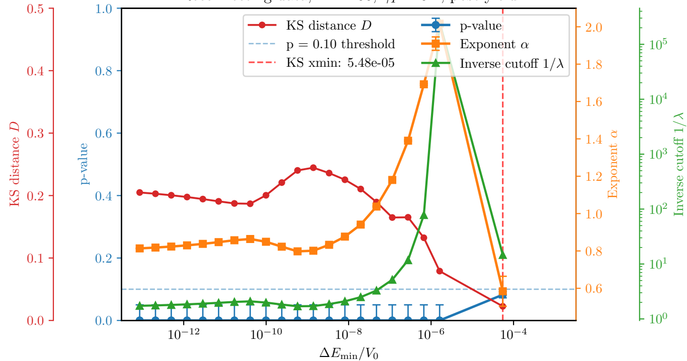
Reconnecting data, L = 200 , \gamma_T = 5.1 , post-yield
