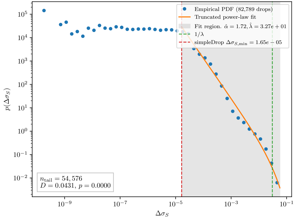
Reconnecting, L = 200 , \gamma_T = 5.1
