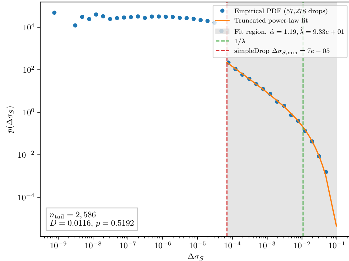
Non-reconnecting, L = 250 , 10 samples
