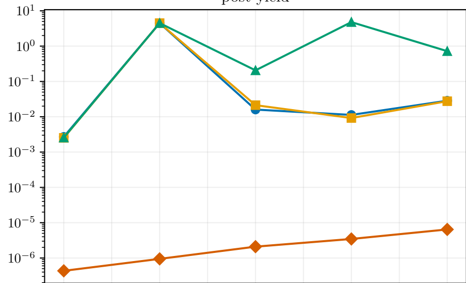
Power-law cutoff and tail support (6 complete seeds per L )
