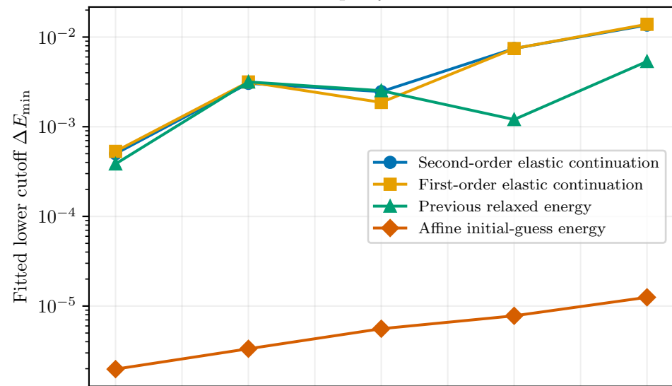
Power-law cutoff and tail support (6 complete seeds per L )
