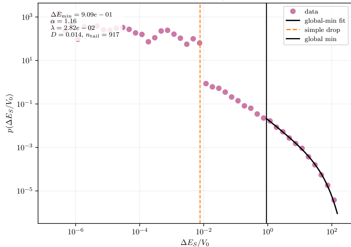
Stress-corrected \Delta E_S ; post-yield; L = 250
