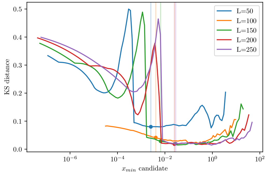
First-order elastic continuation - post-yield Per-size simpleDrop xmin (vertical lines)
