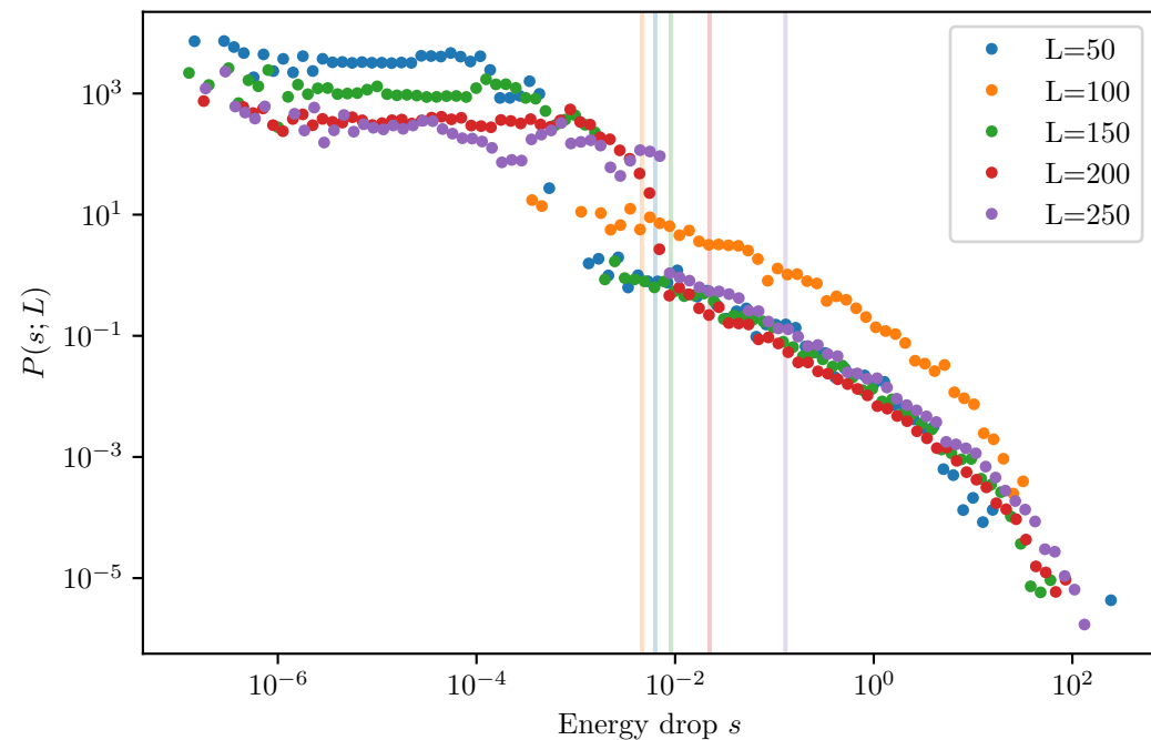
Second-order elastic continuation - post-yield Per-size simpleDrop xmin (vertical lines)
