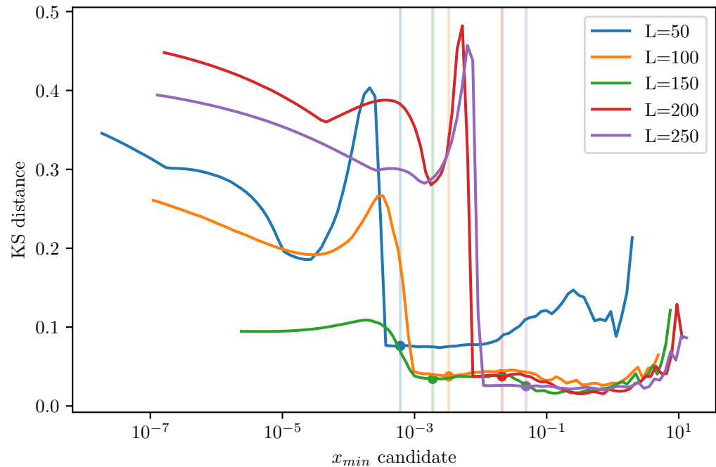
Second-order elastic continuation - pre-yield Per-size simpleDrop xmin (vertical lines)
