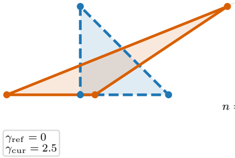
distorted current geometry
