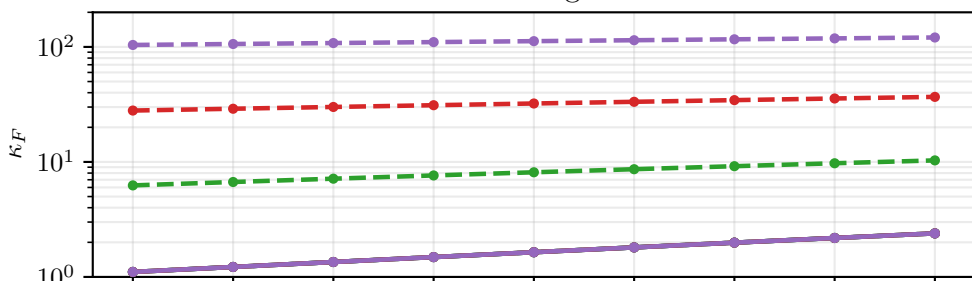
right Cauchy-Green tensor
