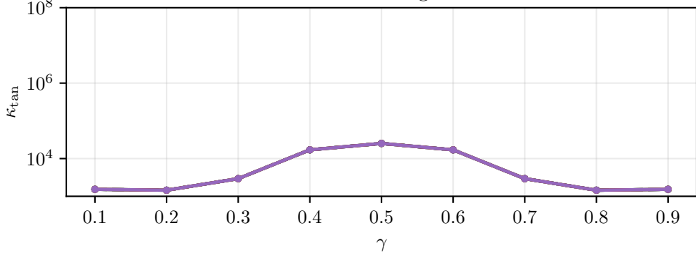
element tangent
