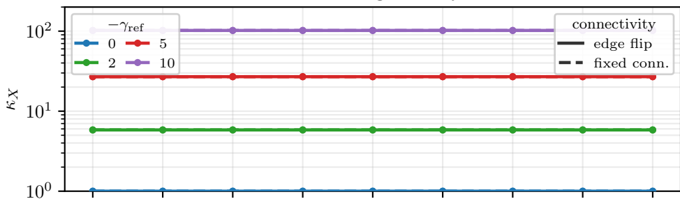
deformation gradient
