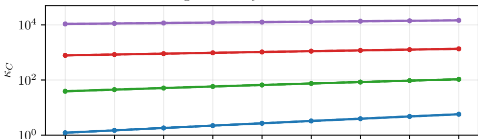
constitutive tangent
