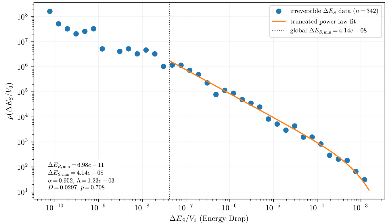
edgeFlip: post-yield \Delta E_R -classified irreversible \Delta E_S
