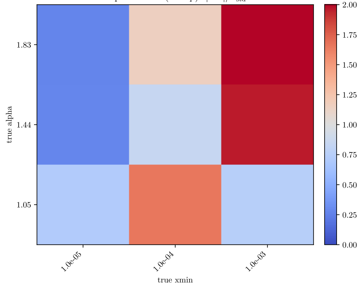
Alpha z-score (max p ): |\Delta\alpha|/\alpha_{\text{std}}
