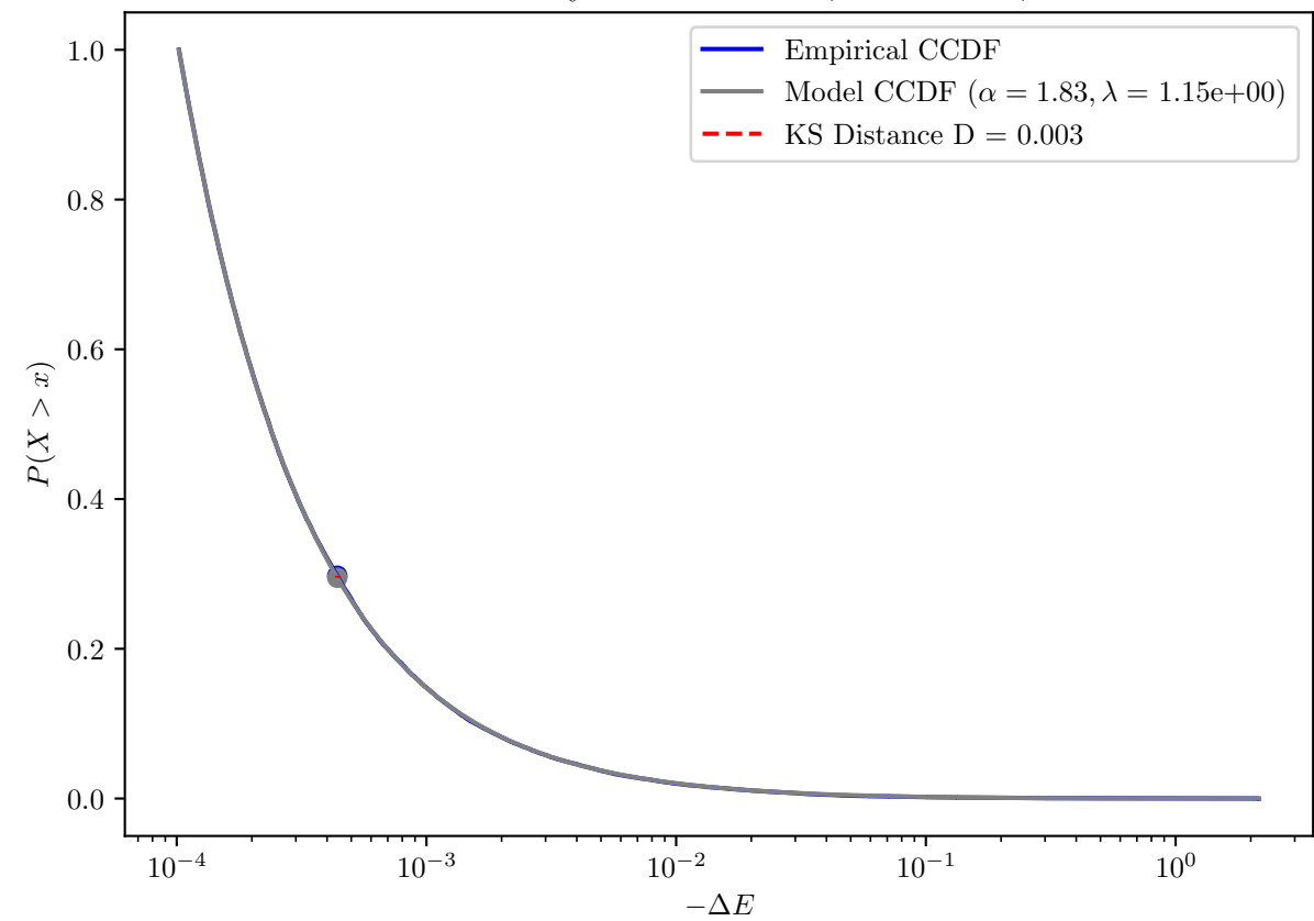
KS Distance E_{\min}=1.02\text{e-}04 Synthetic: \alpha = 1.8, \lambda = 1\text{e} + 00, E_{\min} = 1.00\text{e} - 04
