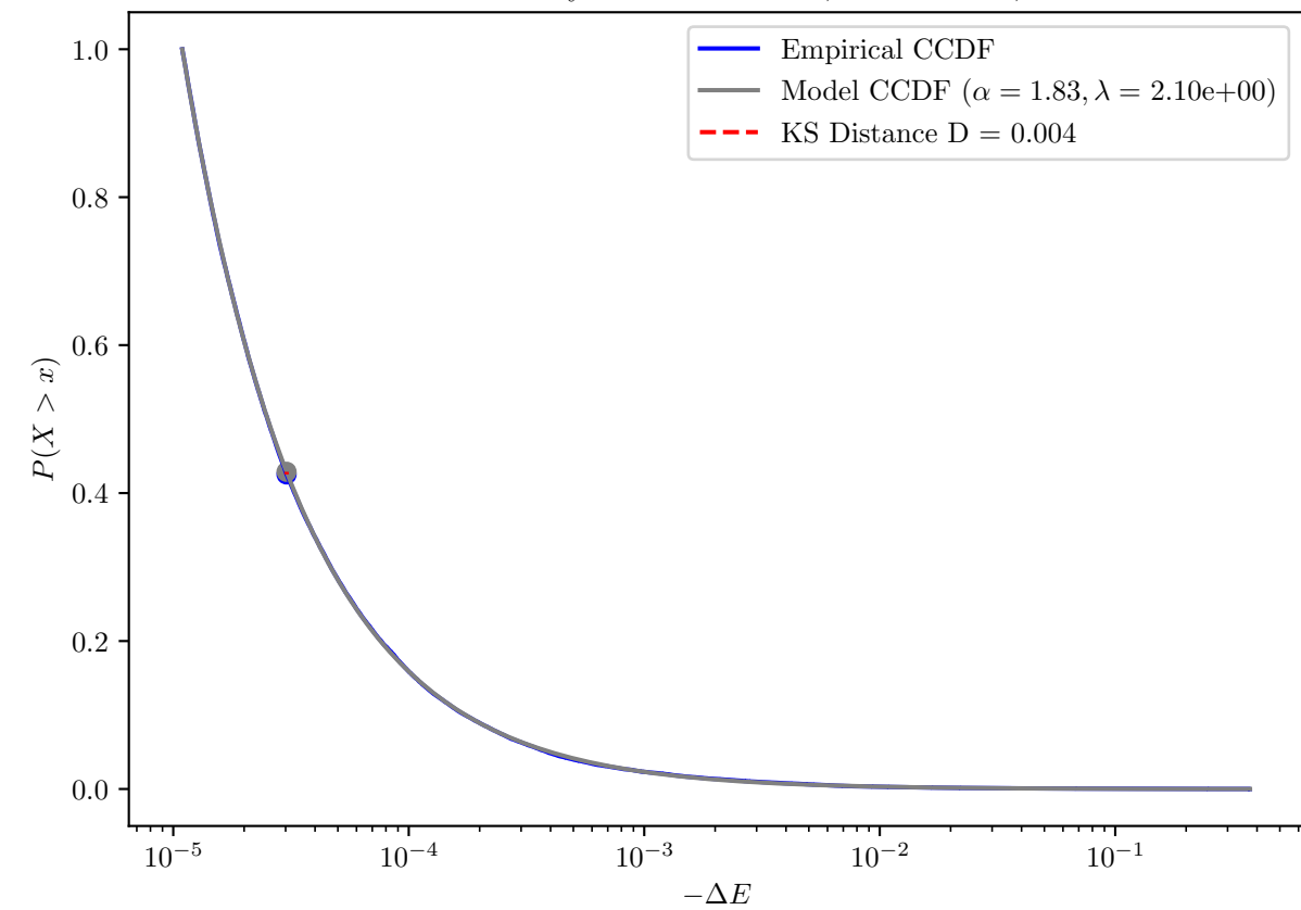
KS Distance E_{\min}=1.09\text{e-}05 Synthetic: \alpha = 1.8, \lambda = 1\text{e} + 00, E_{\min} = 1.00\text{e} - 05
