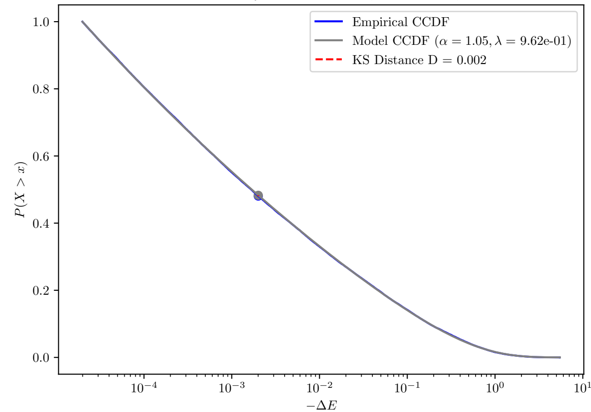
KS Distance E_{\min}=1.99\text{e-}05 Synthetic: \alpha = 1.1, \lambda = 1\text{e} + 00, E_{\min} = 1.00\text{e} - 05
