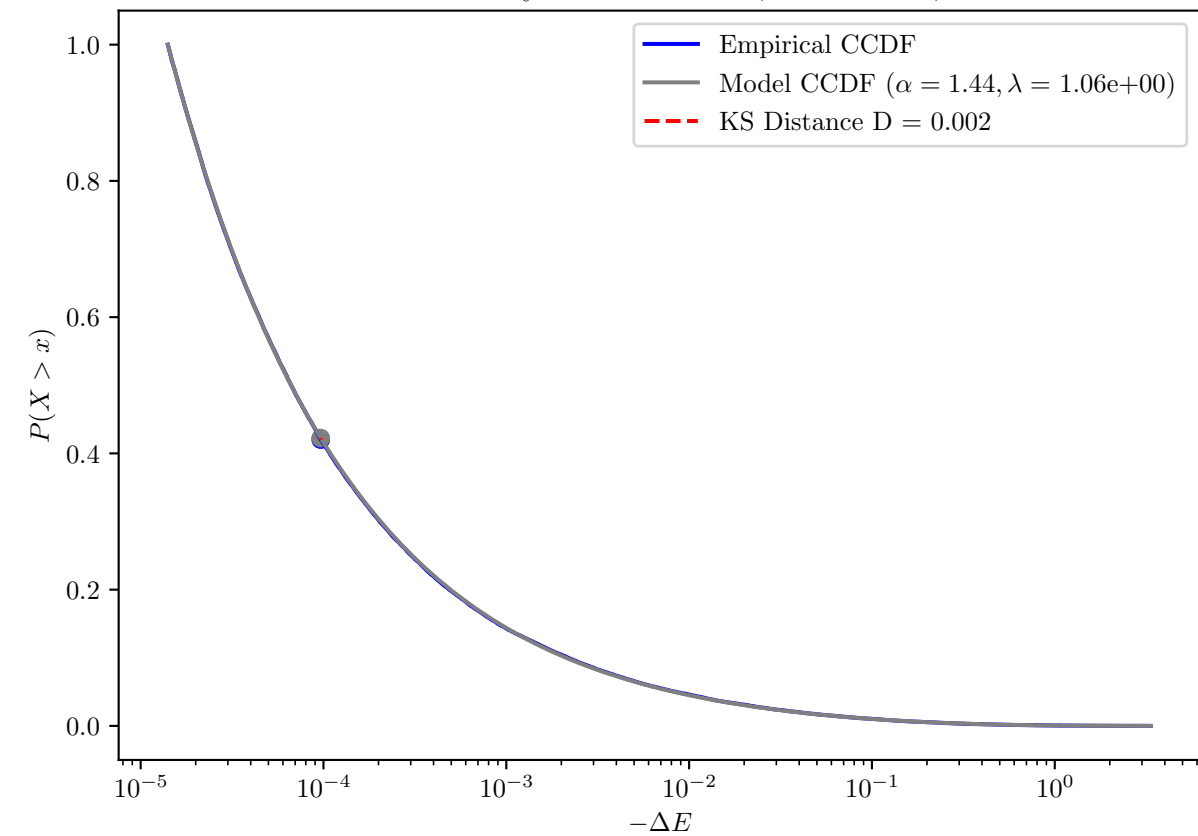
KS Distance E_{\min}=1.41\text{e-}05 Synthetic: \alpha = 1.4, \lambda = 1\text{e} + 00, E_{\min} = 1.00\text{e} - 05
