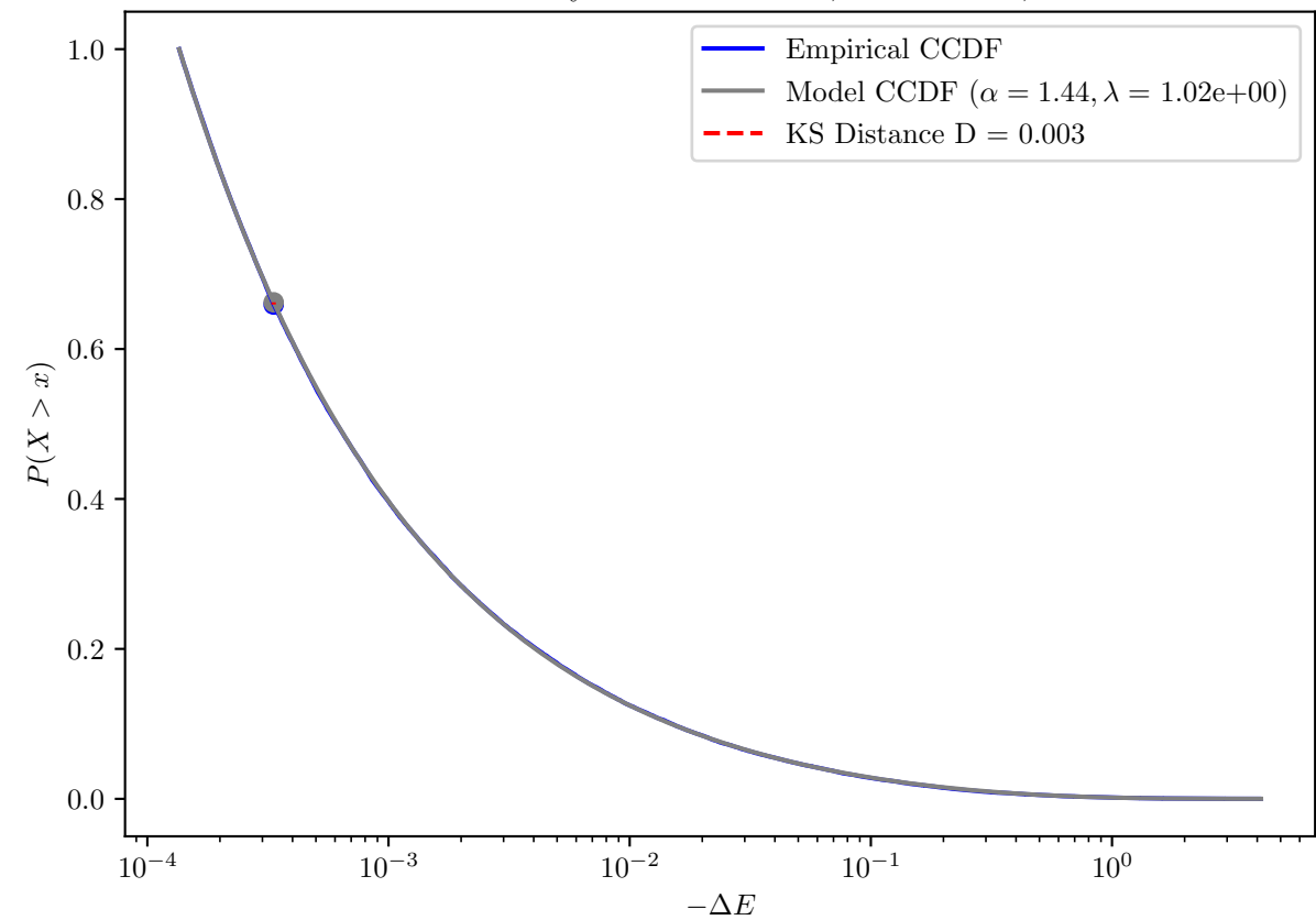
KS Distance E_{\min}=1.35\text{e-}04 Synthetic: \alpha = 1.4, \lambda = 1\text{e} + 00, E_{\min} = 1.00\text{e} - 04
