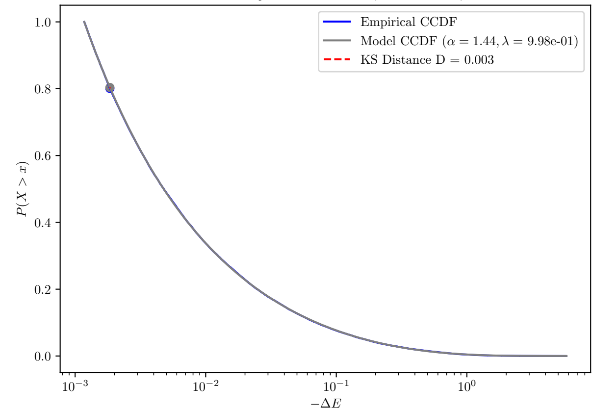
KS Distance E_{\min}=1.18\text{e-}03 Synthetic: \alpha = 1.4, \lambda = 1\text{e} + 00, E_{\min} = 1.00\text{e} - 03
