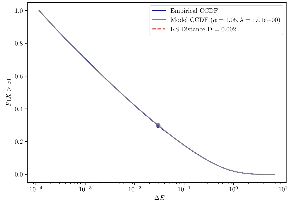
KS Distance E_{\min}=1.17\text{e-}04 Synthetic: \alpha = 1.1, \lambda = 1\text{e} + 00, E_{\min} = 1.00\text{e} - 04
