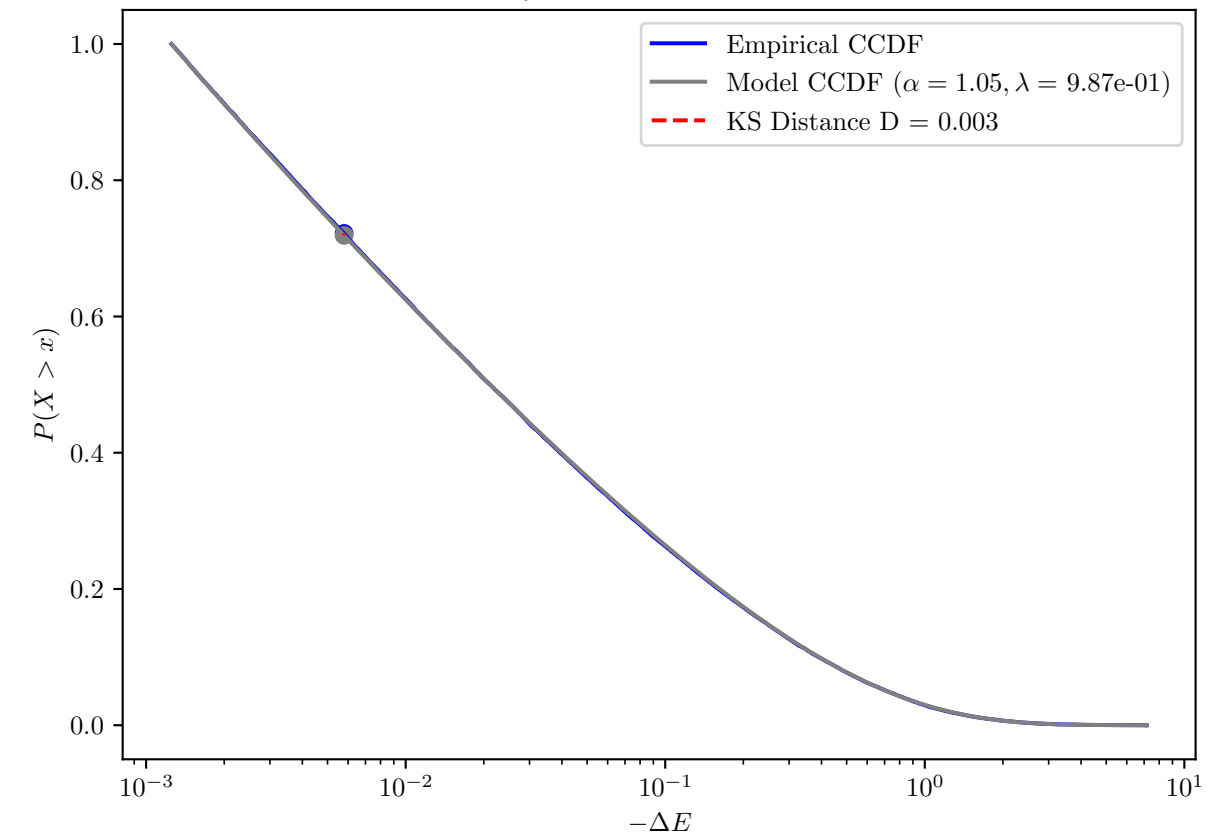
KS Distance E_{\min}=1.25\text{e-}03 Synthetic: \alpha = 1.1, \lambda = 1\text{e} + 00, E_{\min} = 1.00\text{e} - 03
