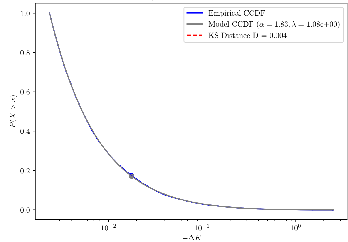
KS Distance E_{\min}=2.35\text{e-}03 Synthetic: \alpha = 1.8, \lambda = 1\text{e} + 00, E_{\min} = 1.00\text{e} - 03
