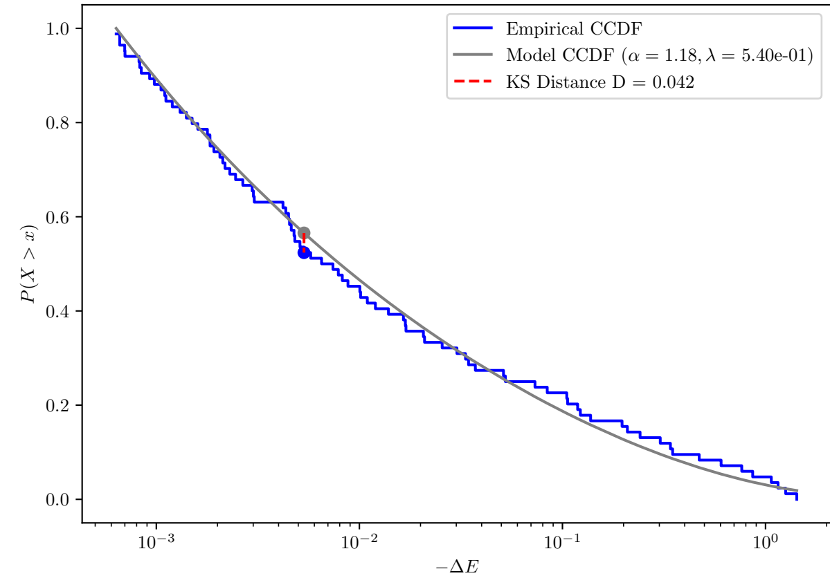
KS Distance E_{\min}=6.34e-04 Synthetic: \alpha = 1.1, \lambda = 1e+00, E_{\min} = 1.00e-03
