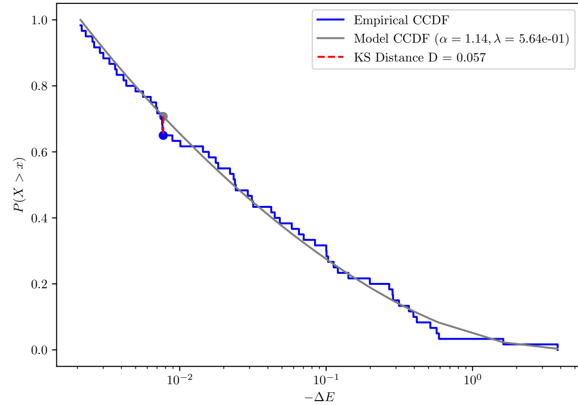
KS Distance E_{\min}=2.10e-03 Synthetic: \alpha = 1.1, \lambda = 1e+00, E_{\min} = 1.00e-04
