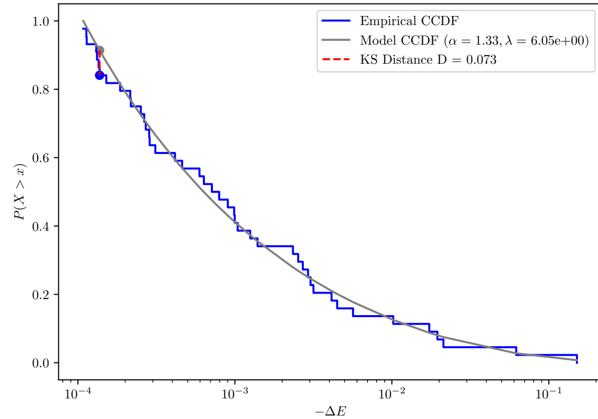
KS Distance E_{\min}=1.08e-04 Synthetic: \alpha = 1.4, \lambda = 1e+00, E_{\min} = 1.00e-04
