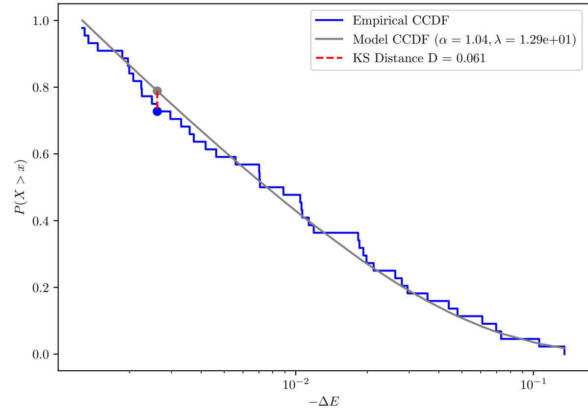
KS Distance E_{\min}=1.26e-03 Synthetic: \alpha = 1.4, \lambda = 1e+00, E_{\min} = 1.00e-03
