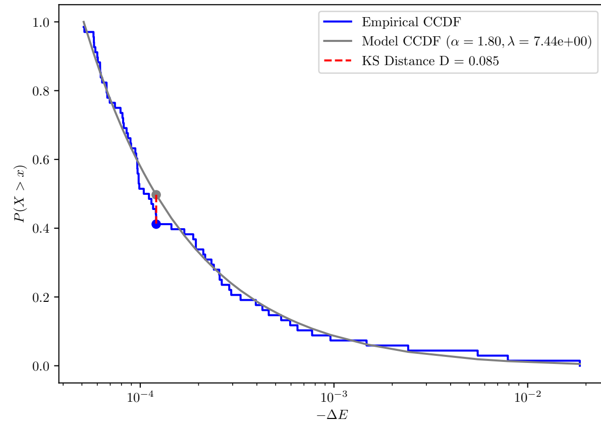
KS Distance E_{\min}=5.11e-05 Synthetic: \alpha = 1.8, \lambda = 1e+00, E_{\min} = 1.00e-04
