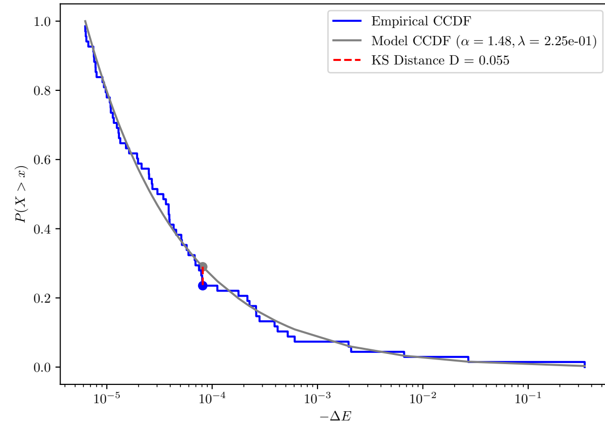
KS Distance E_{\min}=6.24e-06 Synthetic: \alpha = 1.4, \lambda = 1e+00, E_{\min} = 1.00e-05
