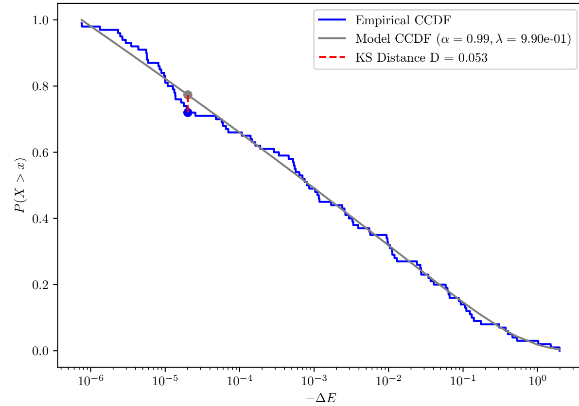
KS Distance E_{\min}=7.54e-07 Synthetic: \alpha = 1.1, \lambda = 1e+00, E_{\min} = 1.00e-05
