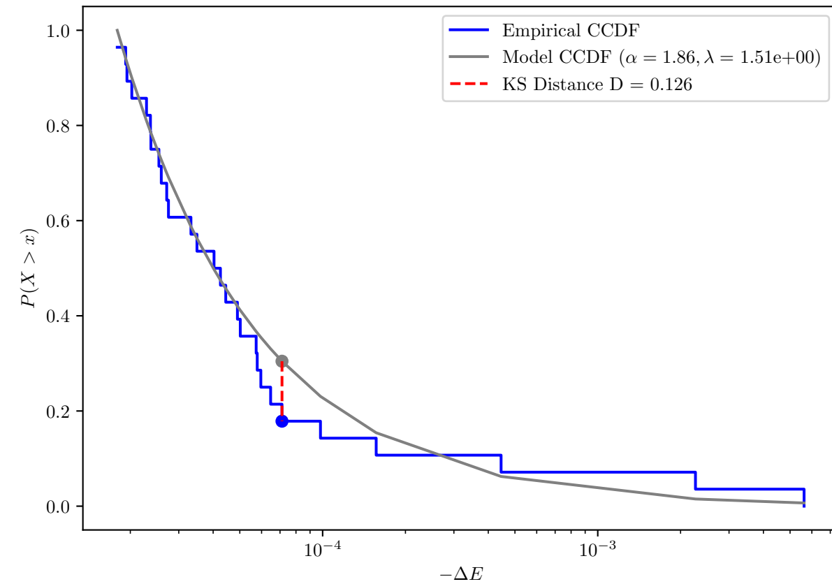
KS Distance E_{\min}=1.79e-05 Synthetic: \alpha = 1.8, \lambda = 1e+00, E_{\min} = 1.00e-05
