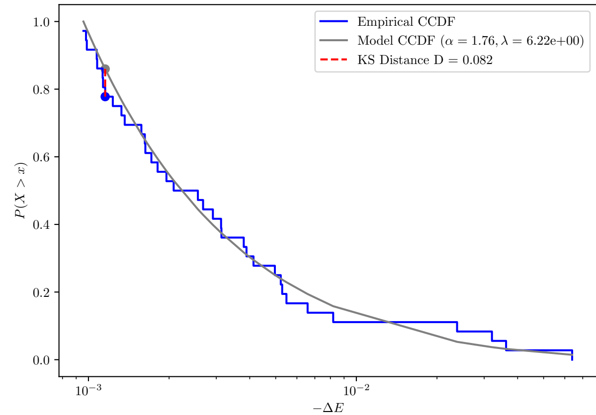
KS Distance E_{\min}=9.58e-04 Synthetic: \alpha = 1.8, \lambda = 1e+00, E_{\min} = 1.00e-03
