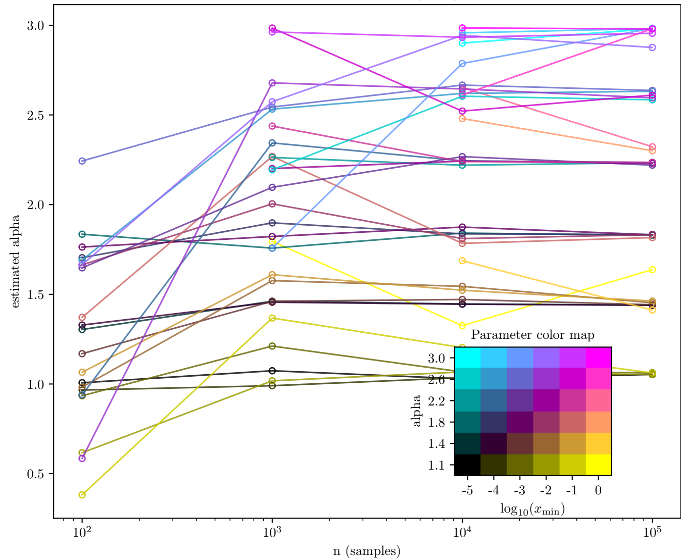
alpha estimate vs n (DKS)
