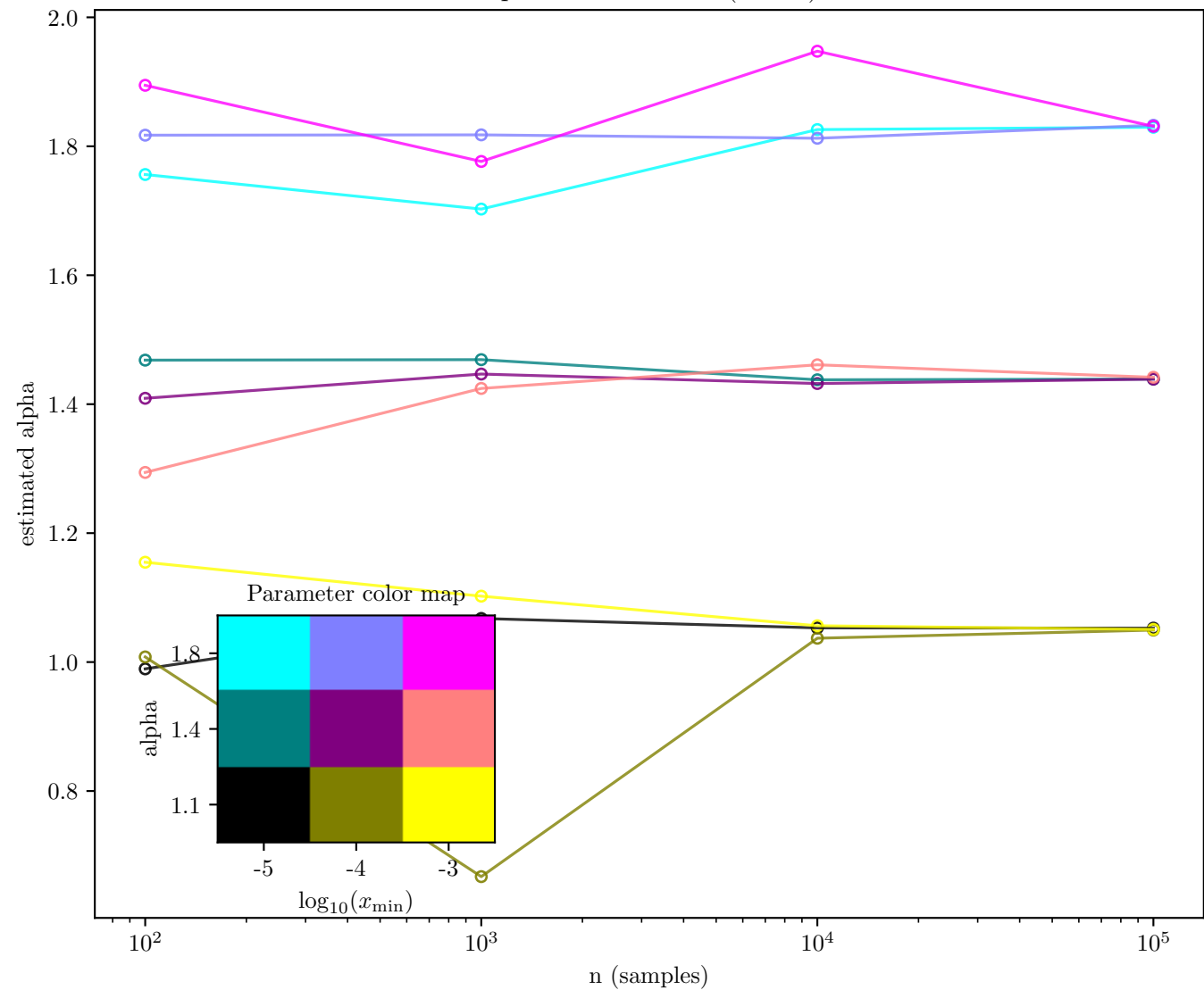
alpha estimate vs n (maxP)
