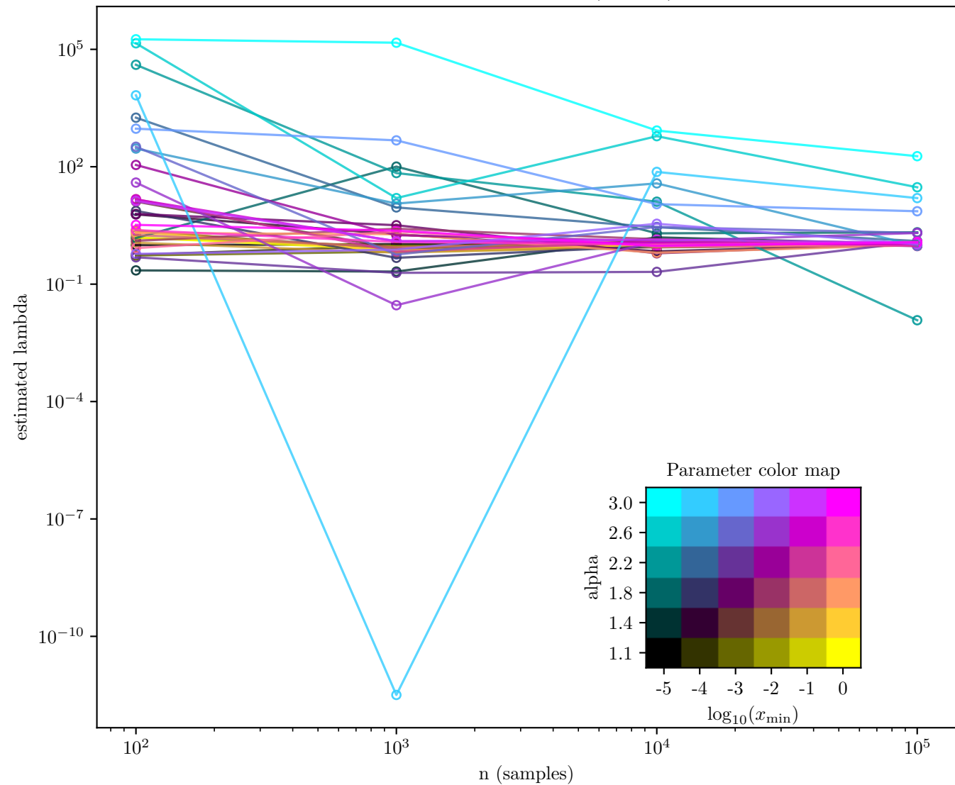
lambda estimate vs n (minKS)
