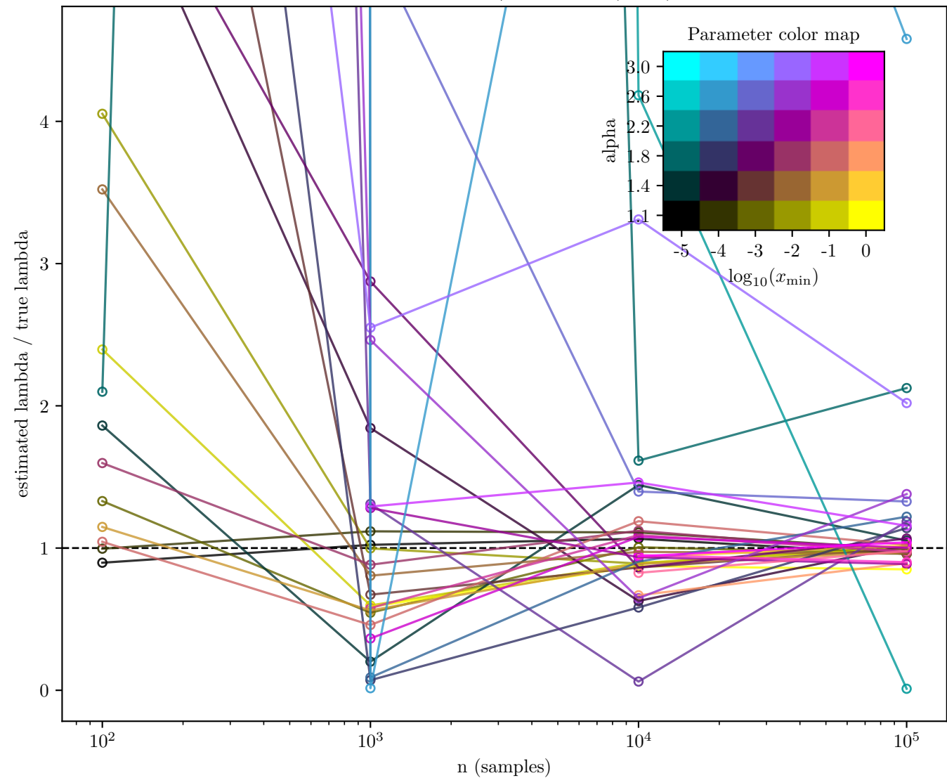
lambda estimate / true vs n (DKS)
