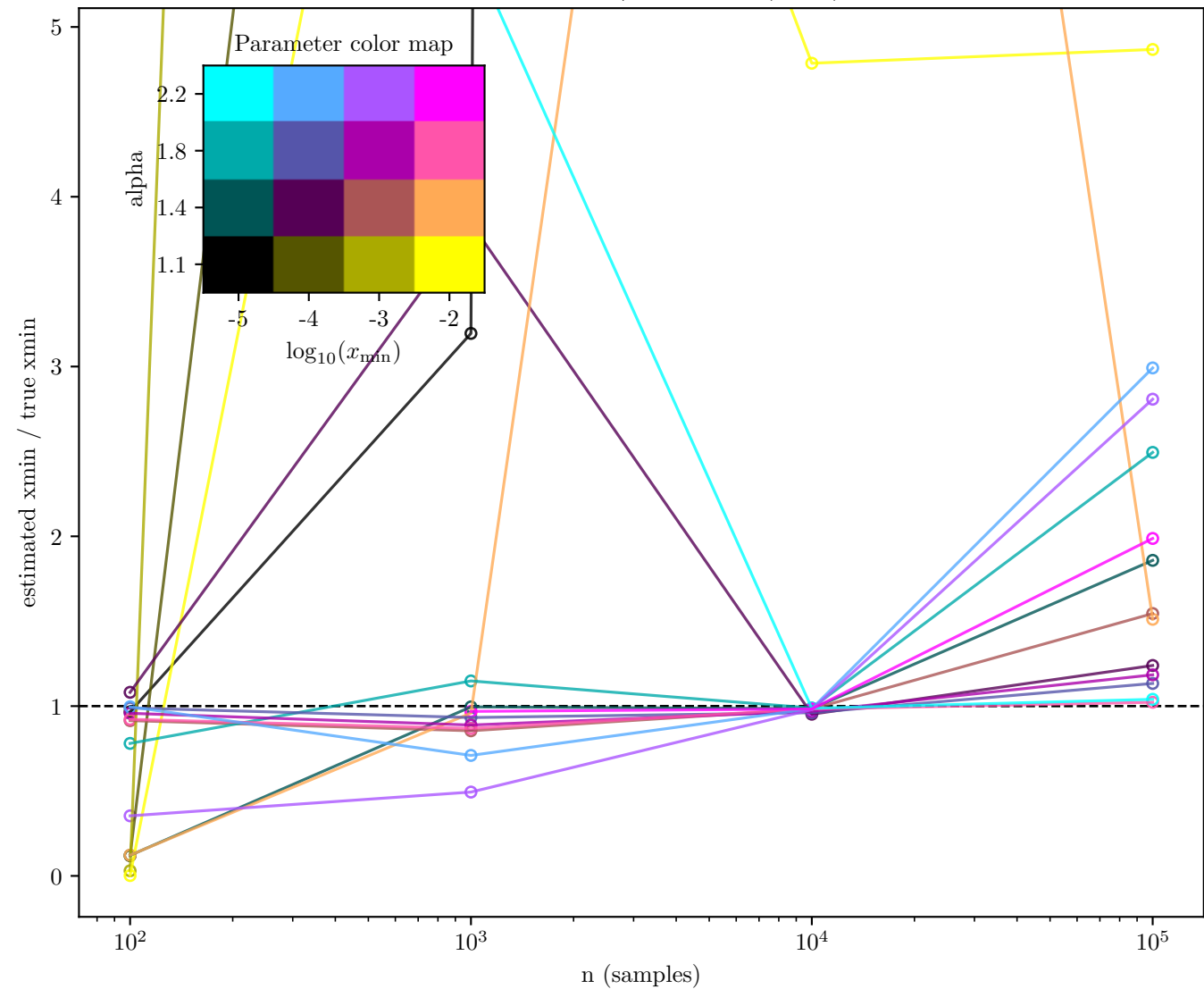
xmin estimate / true vs n (DKS)
