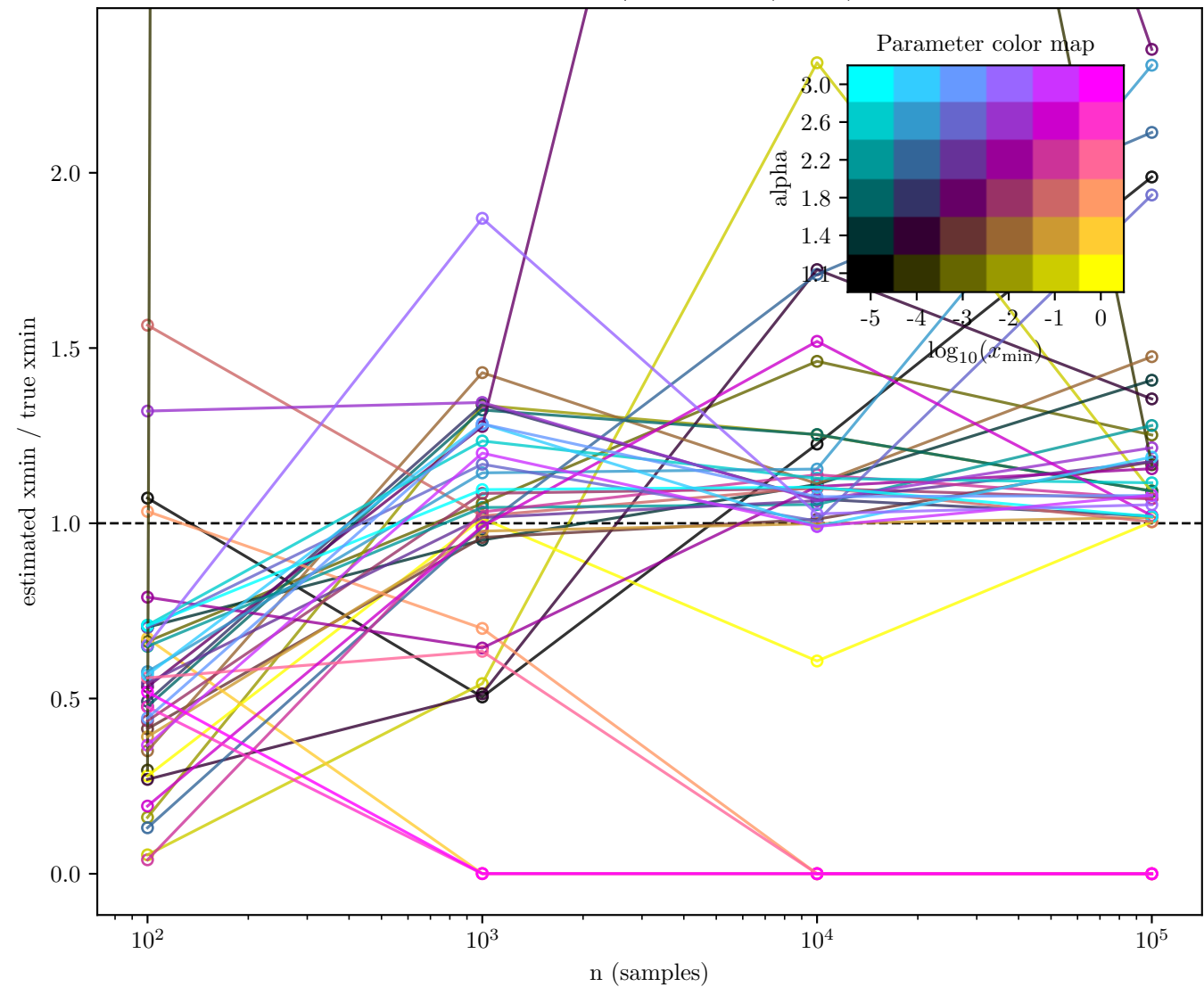
xmin estimate / true vs n (maxP)
