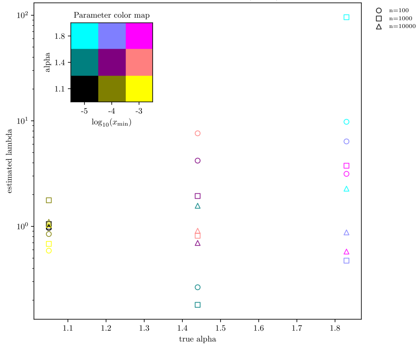
lambda estimate vs true alpha (maxP)
