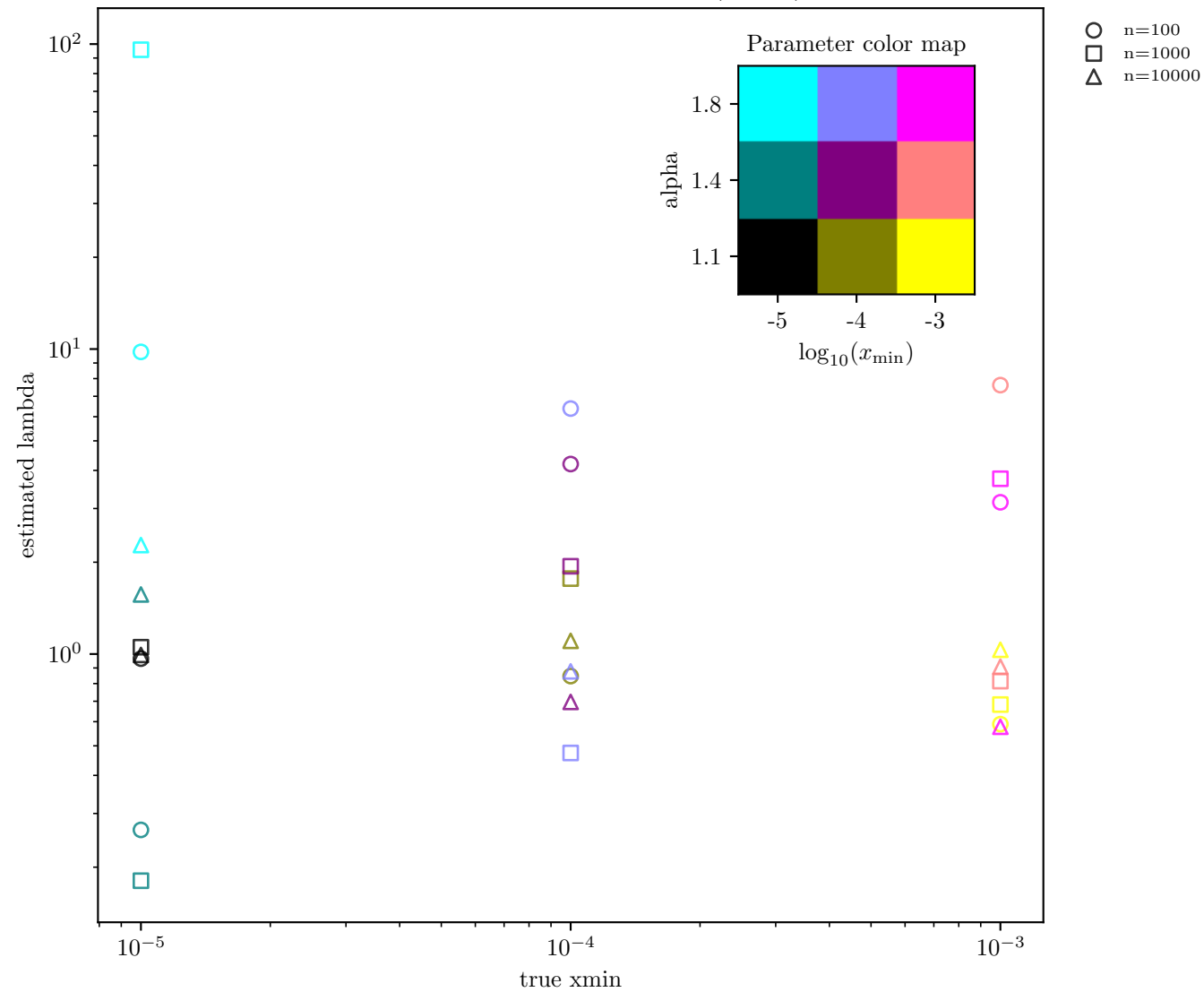
lambda estimate vs true xmin (maxP)
