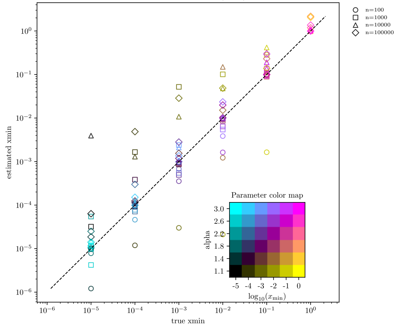
xmin estimate vs true (DKS)
