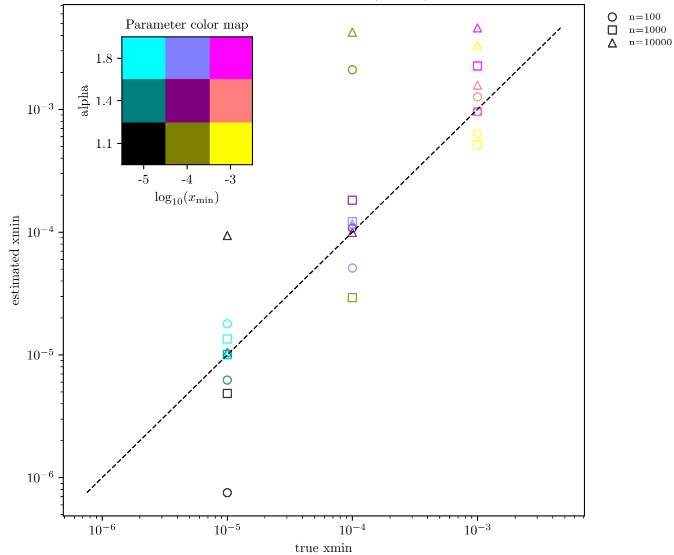
xmin estimate vs true (minKS)
