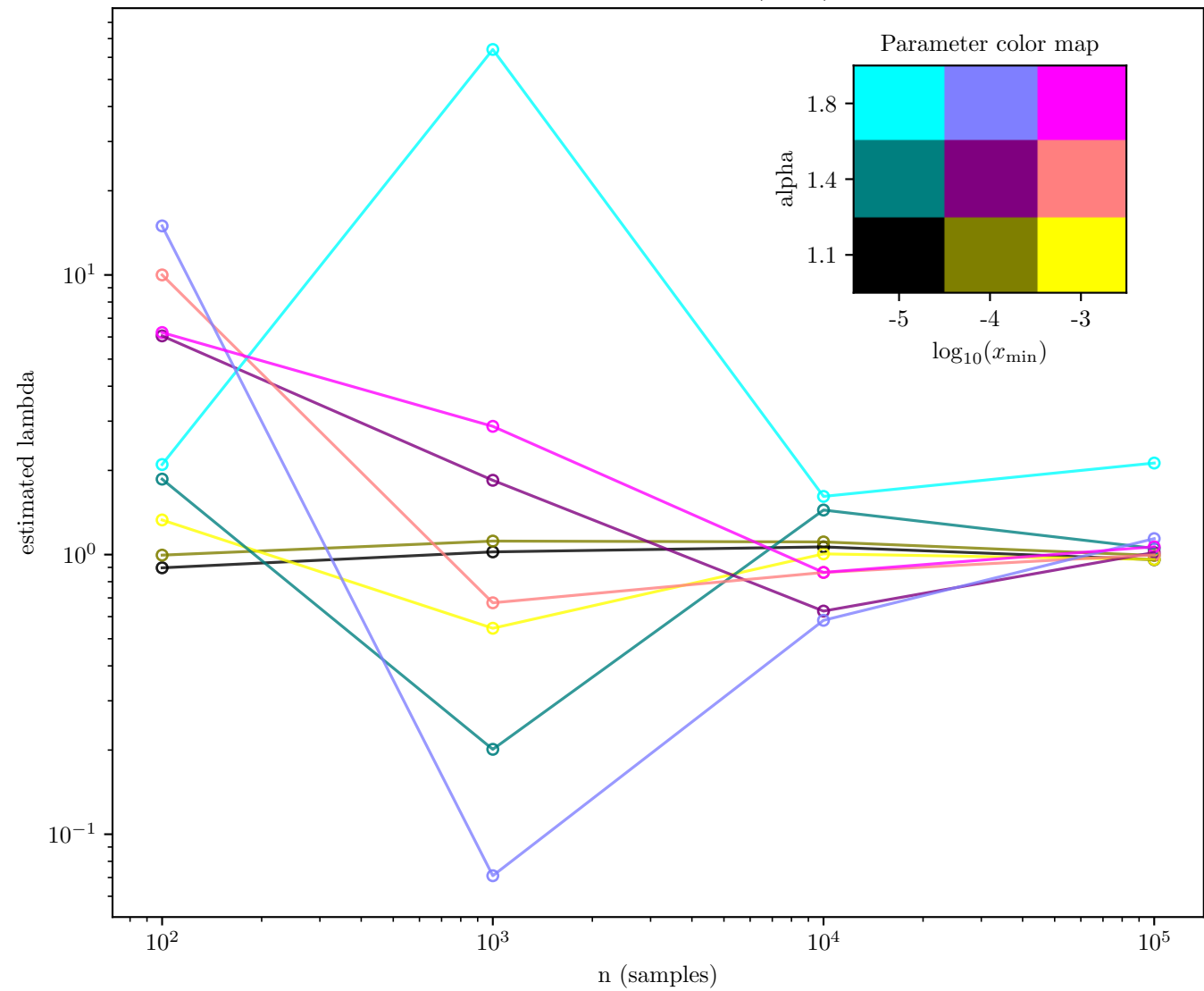
lambda estimate vs n (DKS)
