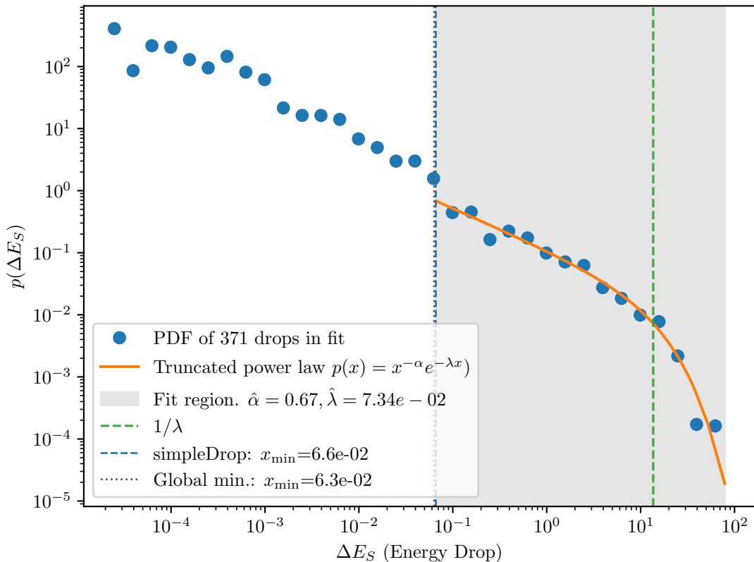
Delaunay reconnecting, L=200, gamma_T=5.1, post-yield
