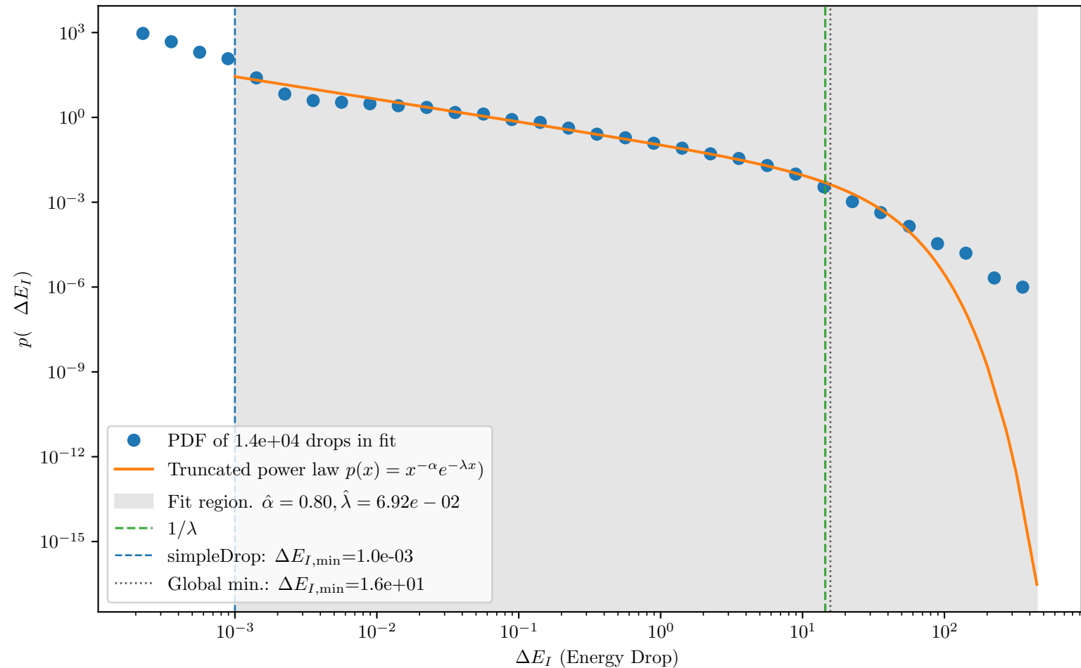
FIRE, L=100: E_I PDF with truncated-power-law fit
