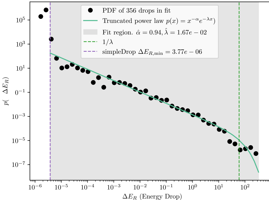
LBFGS, L=200: \Delta E_R PDF with truncated-power-law fit
