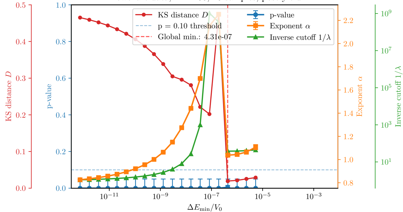
Flowchart data, L = 250 , 10 samples, post-yield
