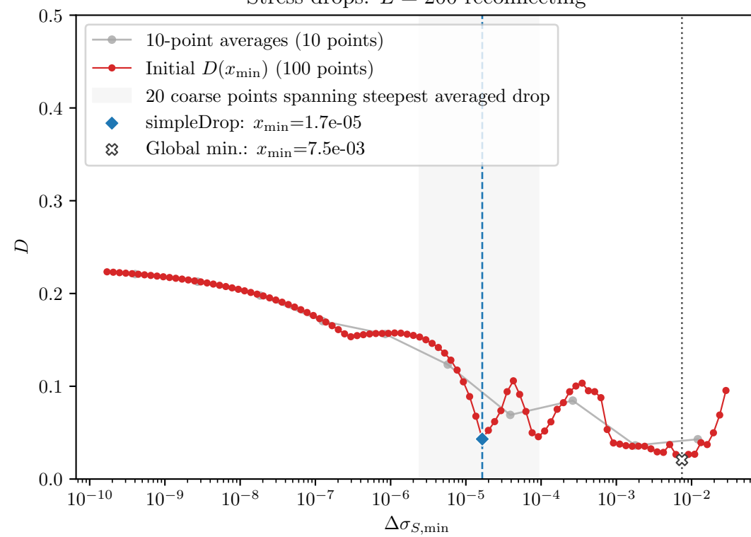
Stress drops: L = 200 reconnecting
