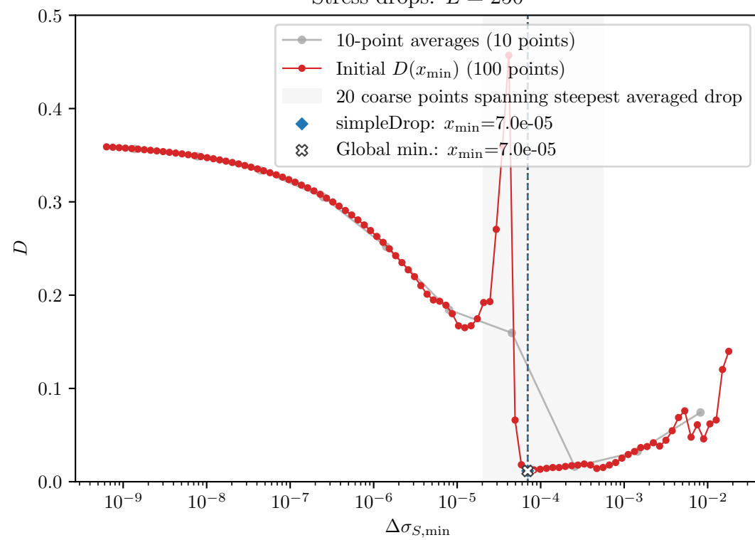
Stress drops: L = 250
