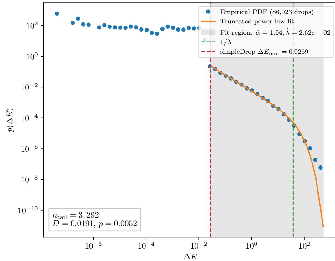
Non-reconnecting, L = 250 , 10 samples
