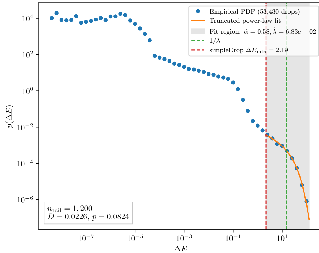
Reconnecting, L = 200, \gamma_T = 5.1
