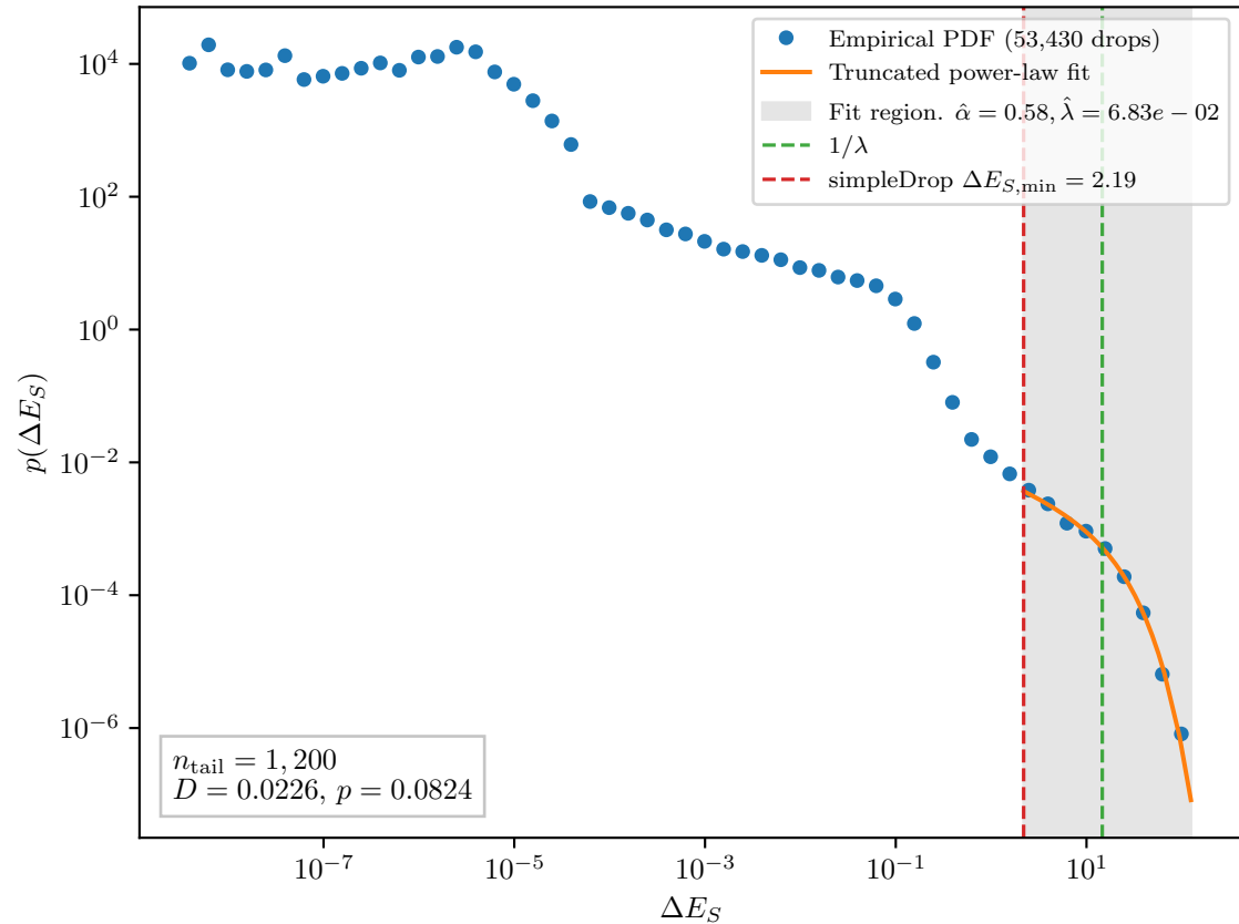
Reconnecting, L = 200 , \gamma_T = 5.1
