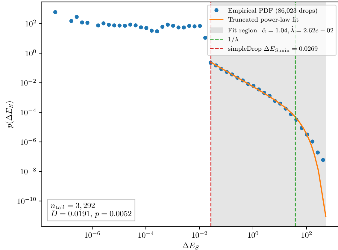
Non-reconnecting, L = 250 , 10 samples
