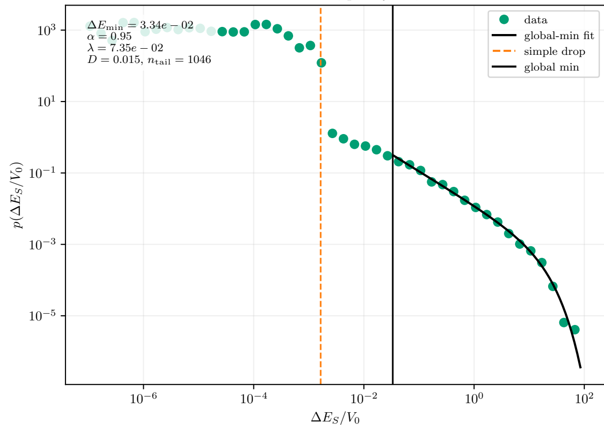
Stress-corrected \Delta E_S ; post-yield; L = 150
