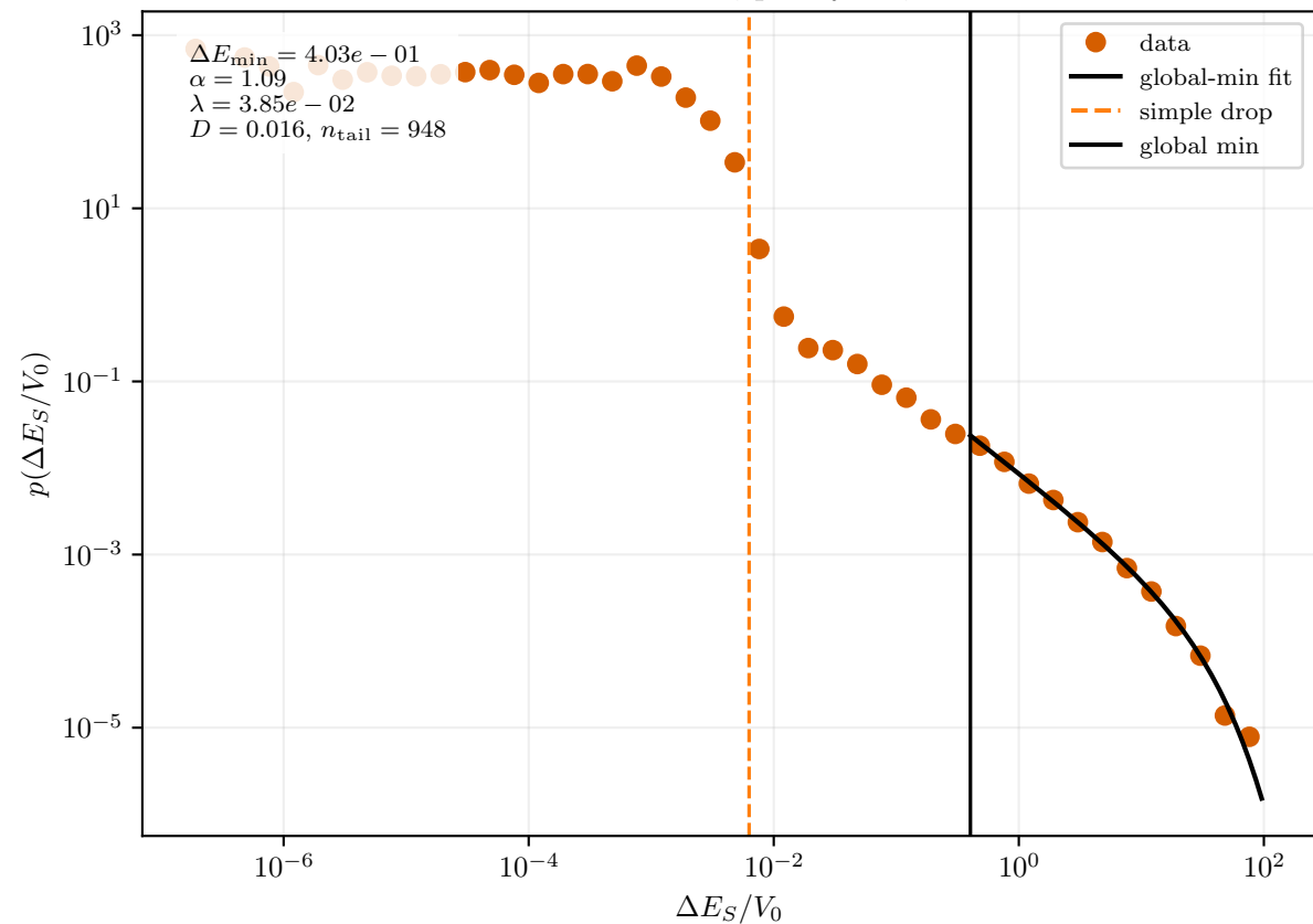
Stress-corrected \Delta E_S ; post-yield; L = 200
