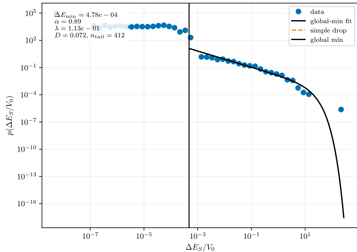
Stress-corrected \Delta E_S ; post-yield; L = 50
