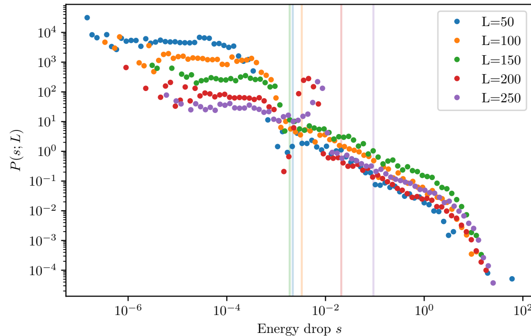
First-order elastic continuation - pre-yield Per-size simpleDrop xmin (vertical lines)
