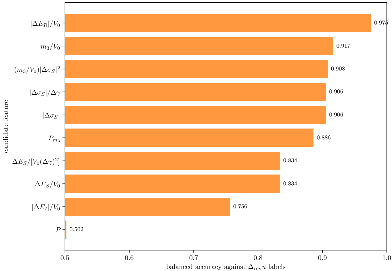
Forward-only Otsu split ranking
